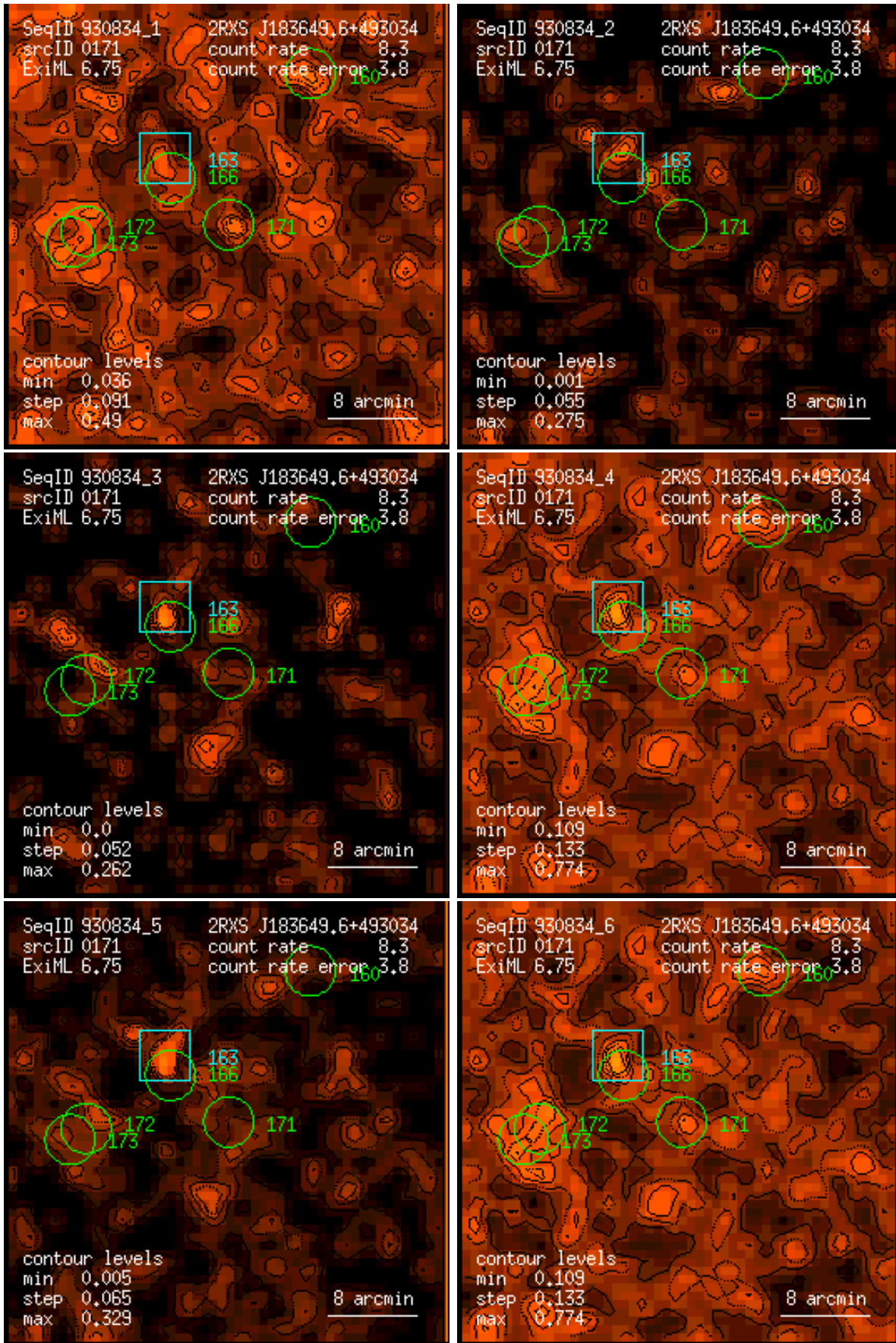
Figure 171: RASS 930834: detection 0171: band rate images, Gaussian filter: (1) PSPC channels 11 – 41, (2) 52 – 90, (3) 91 – 201, (4) 11 – 235, (5) 52 – 201, (6) 11 – 201. Broad band rates in counts/ks. Band rate contour levels in counts/ks/arcmin 2 .
