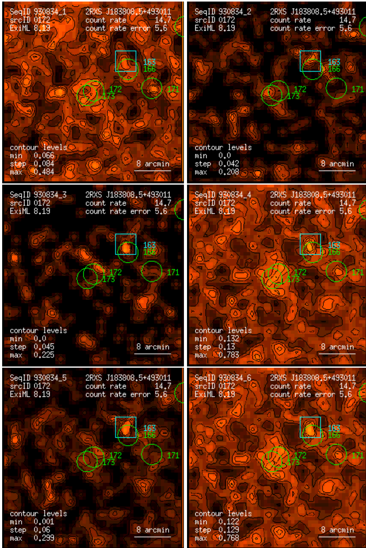
Figure 172: RASS 930834: detection 0172: band rate images, Gaussian filter: (1) PSPC channels 11 – 41, (2) 52 – 90, (3) 91 – 201, (4) 11 – 235, (5) 52 – 201, (6) 11 – 201. Broad band rates in counts/ks. Band rate contour levels in counts/ks/arcmin 2 .
