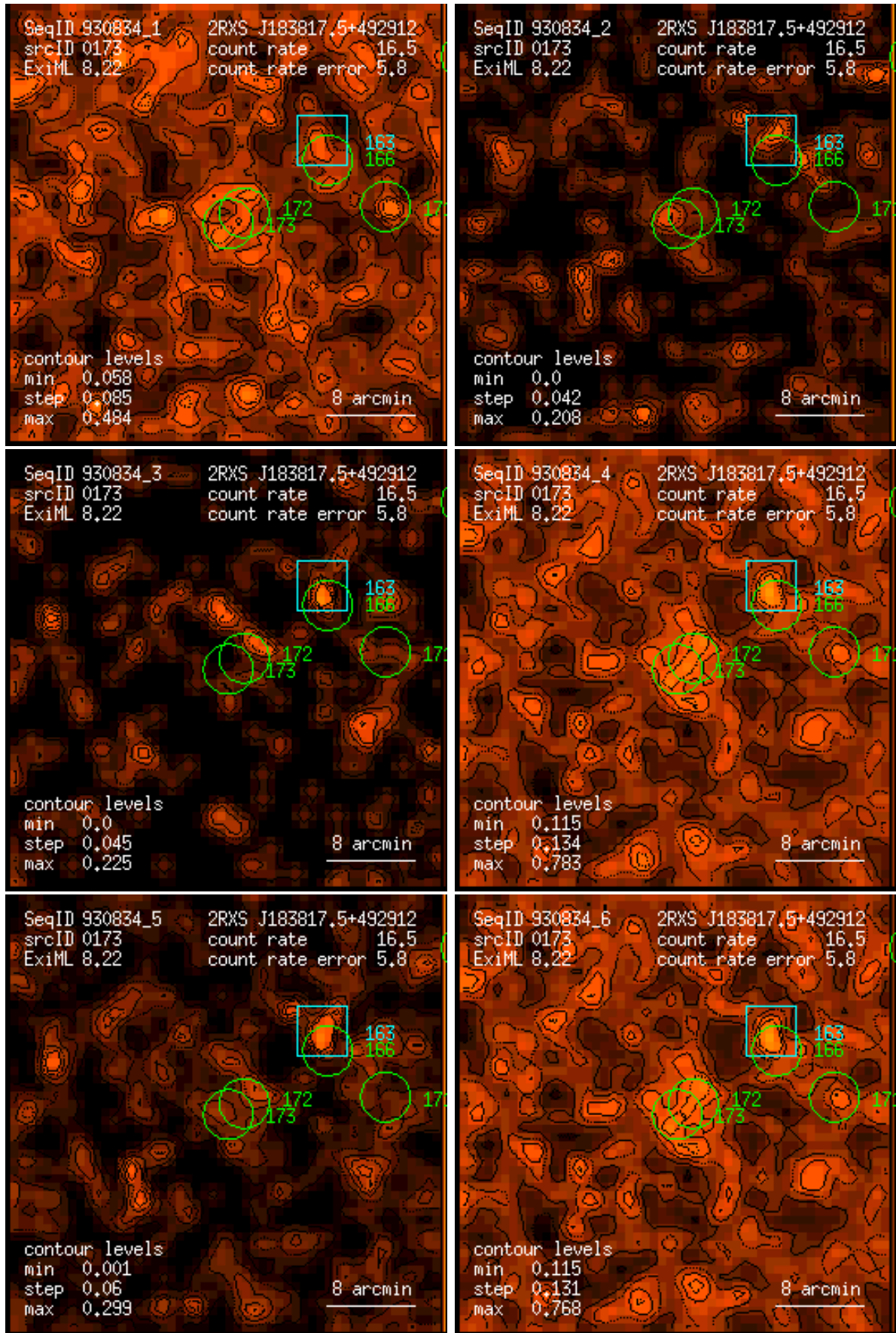
Figure 173: RASS 930834: detection 0173: band rate images, Gaussian filter: (1) PSPC channels 11 – 41, (2) 52 – 90, (3) 91 – 201, (4) 11 – 235, (5) 52 – 201, (6) 11 – 201. Broad band rates in counts/ks. Band rate contour levels in counts/ks/arcmin 2 .
