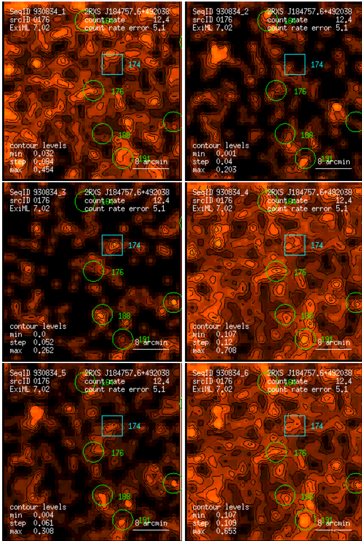
Figure 176: RASS 930834: detection 0176: band rate images, Gaussian filter: (1) PSPC channels 11 – 41, (2) 52 – 90, (3) 91 – 201, (4) 11 – 235, (5) 52 – 201, (6) 11 – 201. Broad band rates in counts/ks. Band rate contour levels in counts/ks/arcmin 2 .
