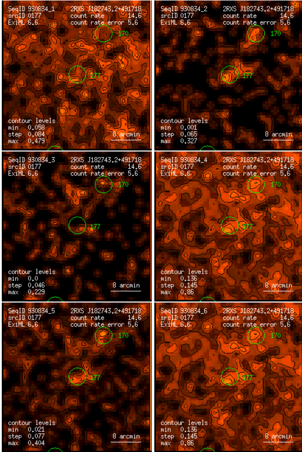
Figure 177: RASS 930834: detection 0177: band rate images, Gaussian filter: (1) PSPC channels 11 – 41, (2) 52 – 90, (3) 91 – 201, (4) 11 – 235, (5) 52 – 201, (6) 11 – 201. Broad band rates in counts/ks. Band rate contour levels in counts/ks/arcmin 2 .
