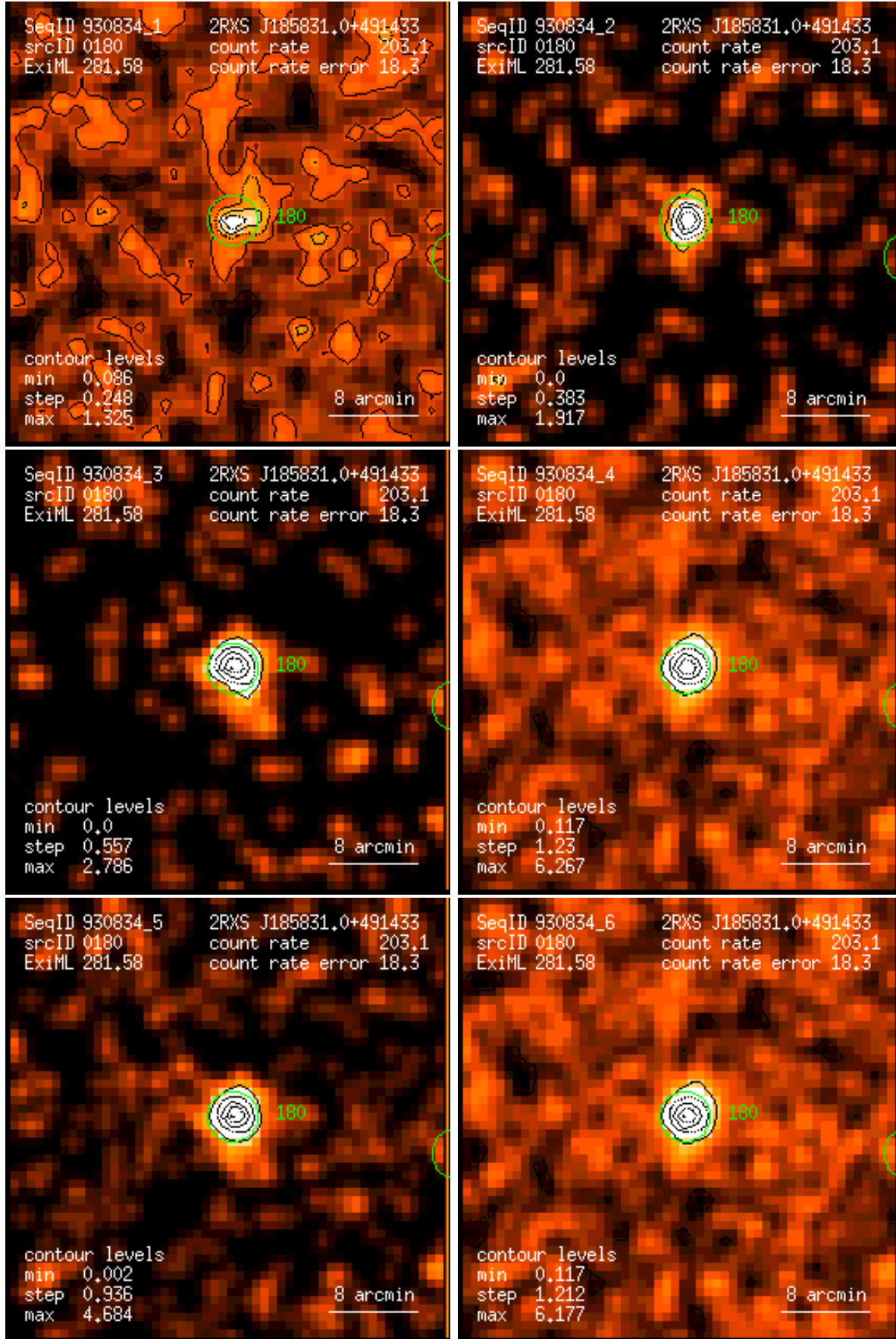
Figure 180: RASS 930834: detection 0180: band rate images, Gaussian filter: (1) PSPC channels 11 – 41, (2) 52 – 90, (3) 91 – 201, (4) 11 – 235, (5) 52 – 201, (6) 11 – 201. Broad band rates in counts/ks. Band rate contour levels in counts/ks/arcmin 2 .
