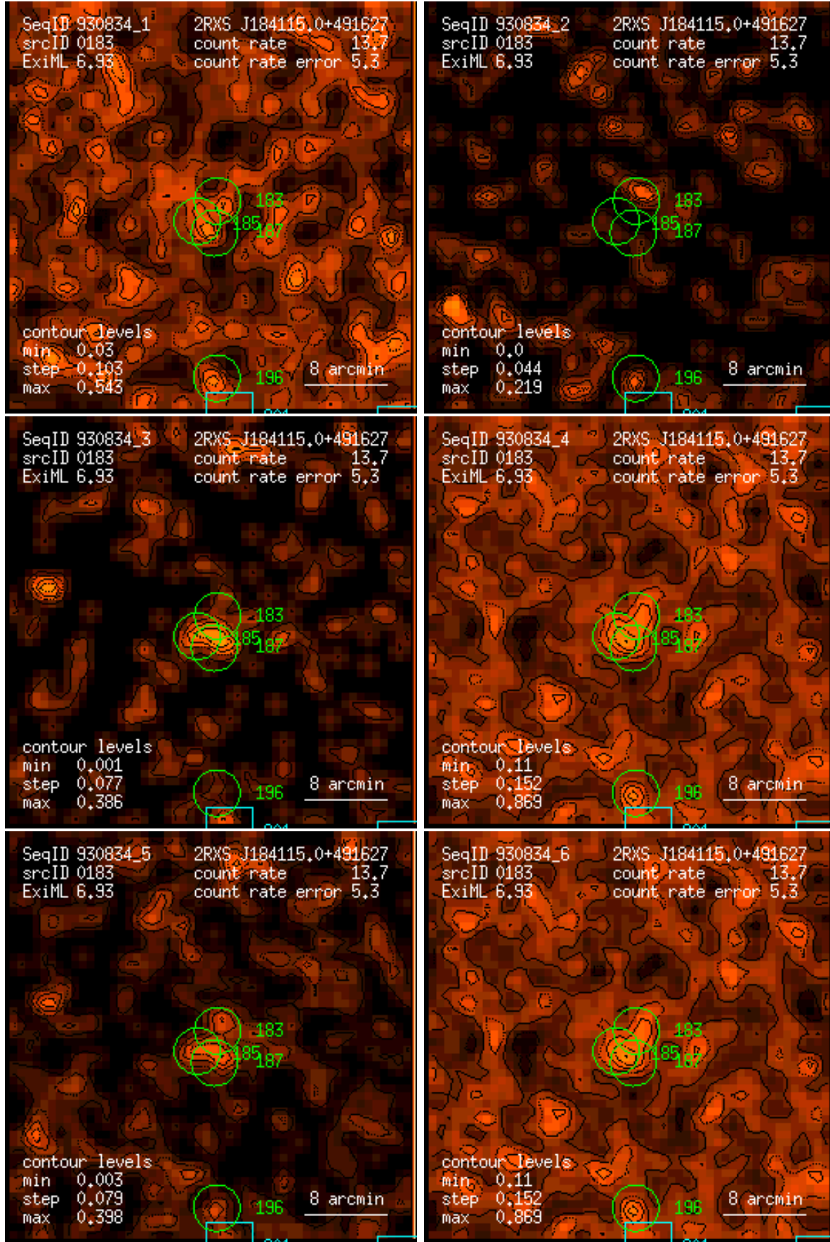
Figure 183: RASS 930834: detection 0183: band rate images, Gaussian filter: (1) PSPC channels 11 – 41, (2) 52 – 90, (3) 91 – 201, (4) 11 – 235, (5) 52 – 201, (6) 11 – 201. Broad band rates in counts/ks. Band rate contour levels in counts/ks/arcmin 2 .
