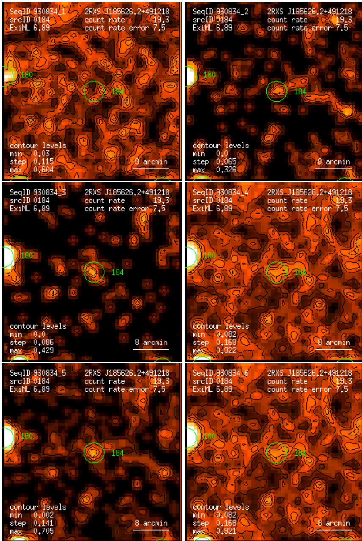
Figure 184: RASS 930834: detection 0184: band rate images, Gaussian filter: (1) PSPC channels 11 – 41, (2) 52 – 90, (3) 91 – 201, (4) 11 – 235, (5) 52 – 201, (6) 11 – 201. Broad band rates in counts/ks. Band rate contour levels in counts/ks/arcmin 2 .
