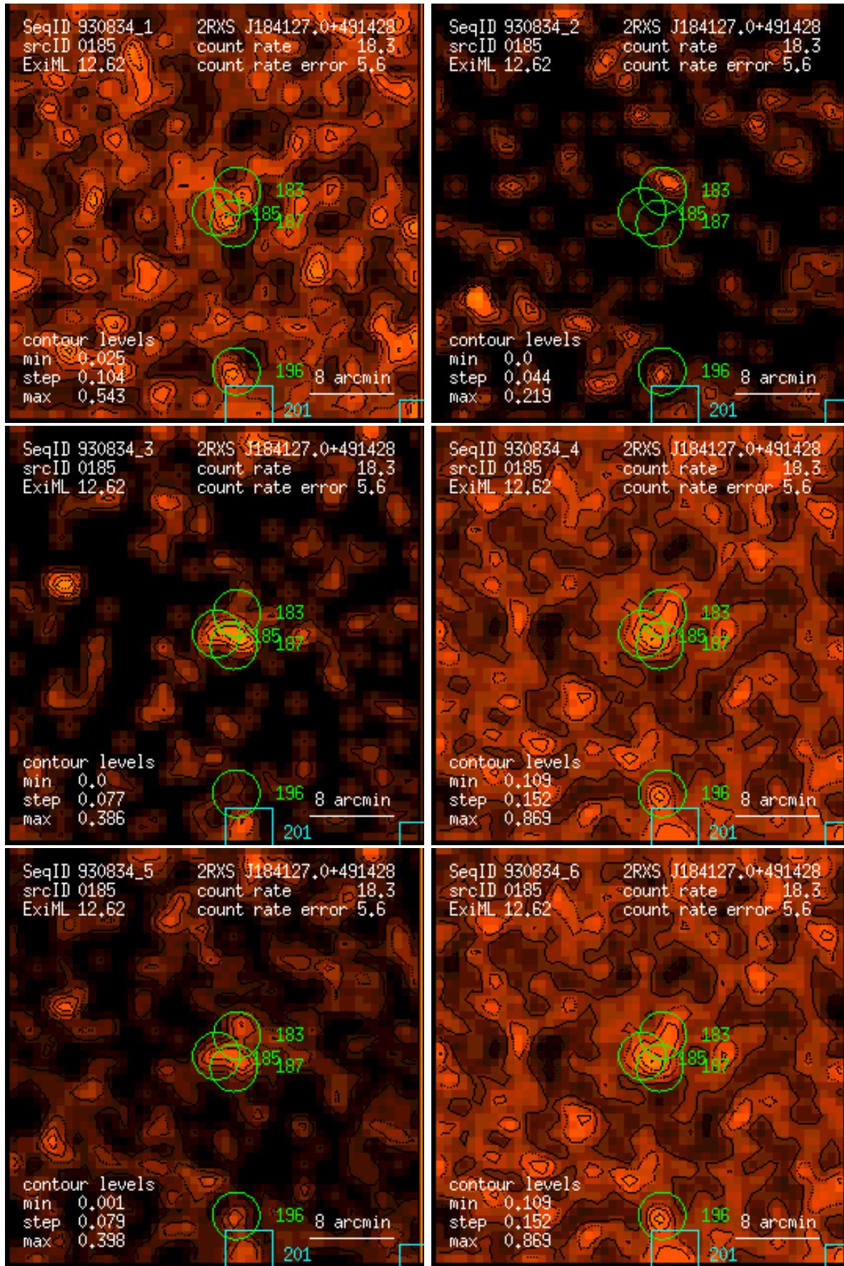
Figure 185: RASS 930834: detection 0185: band rate images, Gaussian filter: (1) PSPC channels 11 – 41, (2) 52 – 90, (3) 91 – 201, (4) 11 – 235, (5) 52 – 201, (6) 11 – 201. Broad band rates in counts/ks. Band rate contour levels in counts/ks/arcmin 2 .
