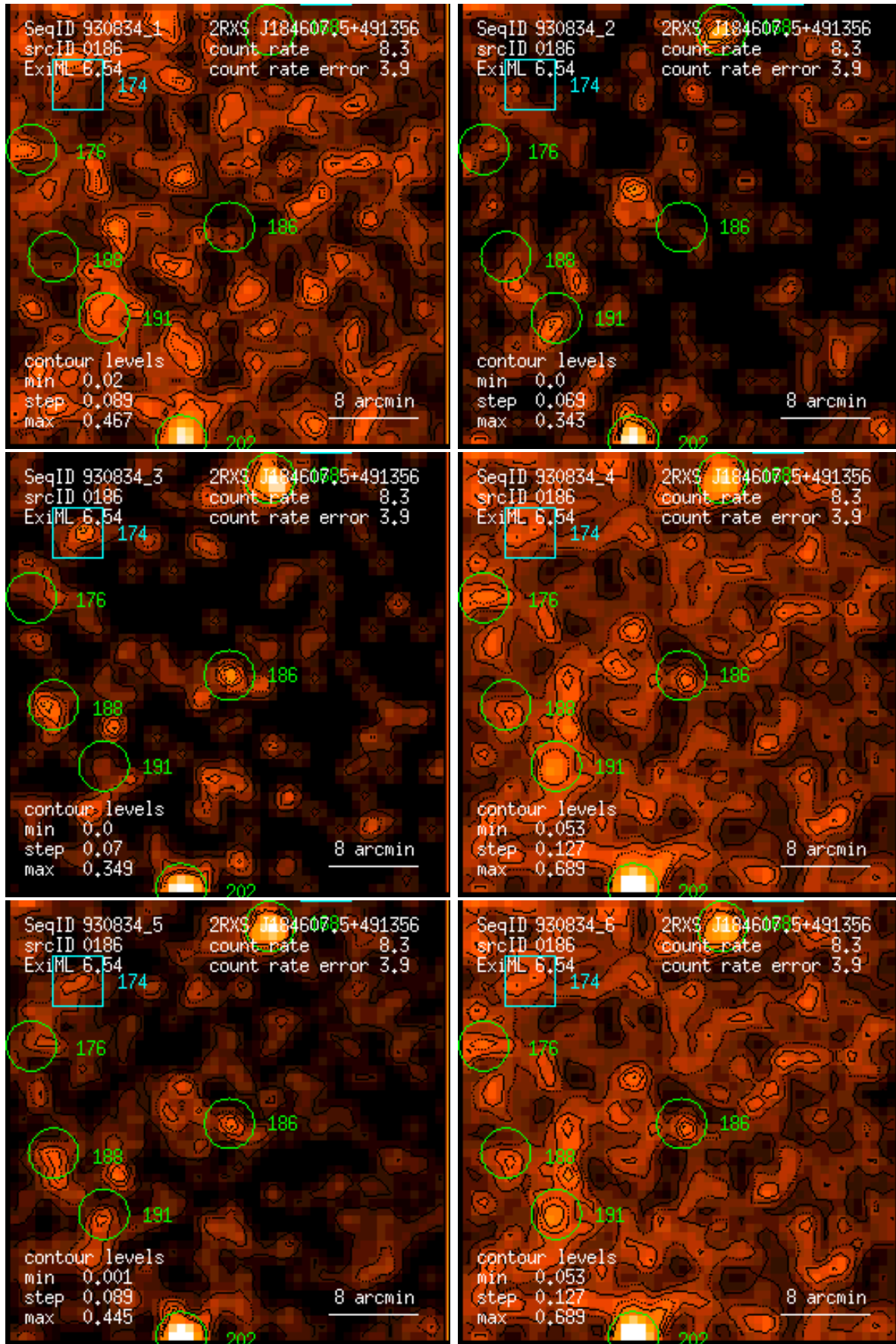
Figure 186: RASS 930834: detection 0186: band rate images, Gaussian filter: (1) PSPC channels 11 – 41, (2) 52 – 90, (3) 91 – 201, (4) 11 – 235, (5) 52 – 201, (6) 11 – 201. Broad band rates in counts/ks. Band rate contour levels in counts/ks/arcmin 2 .
