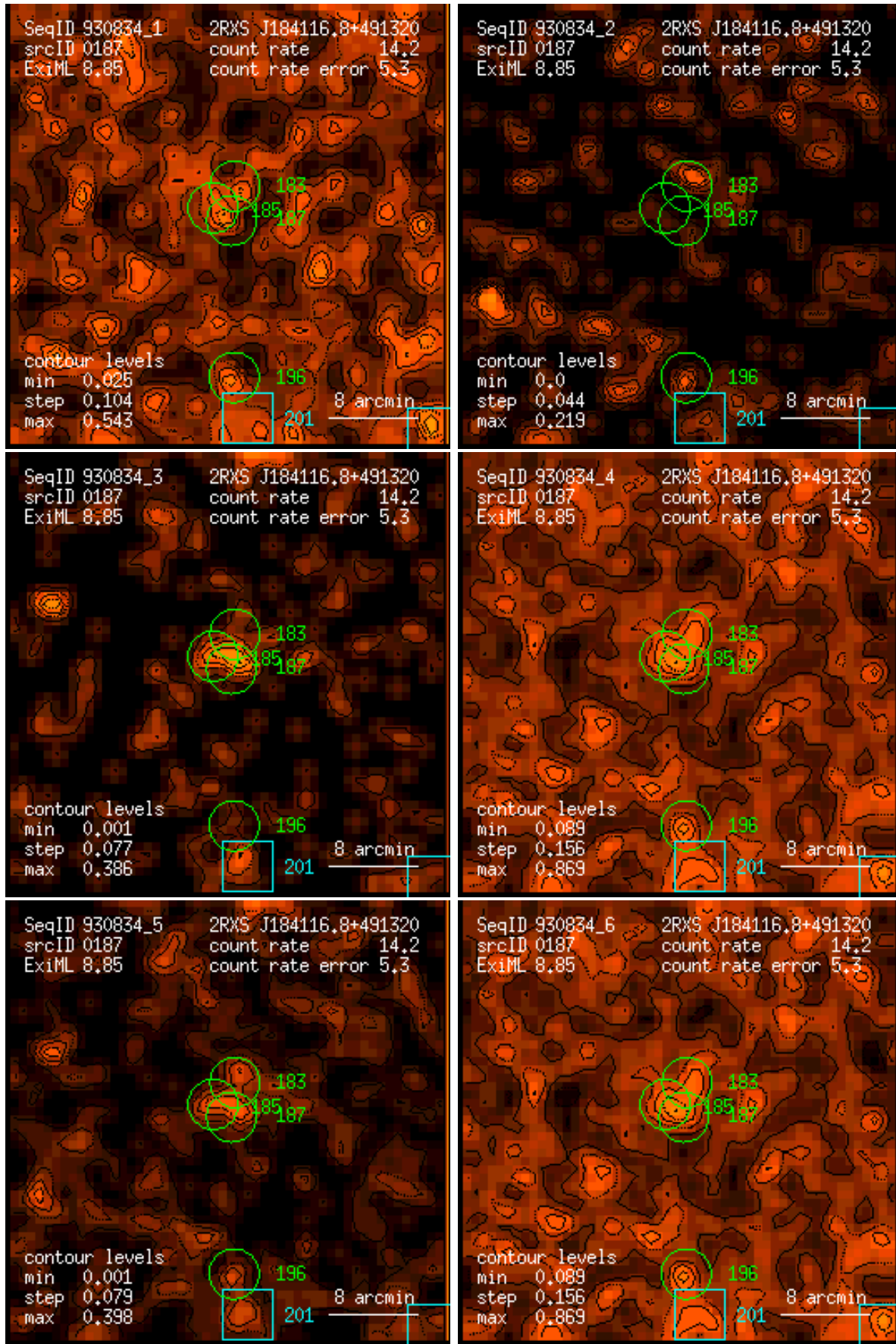
Figure 187: RASS 930834: detection 0187: band rate images, Gaussian filter: (1) PSPC channels 11 – 41, (2) 52 – 90, (3) 91 – 201, (4) 11 – 235, (5) 52 – 201, (6) 11 – 201. Broad band rates in counts/ks. Band rate contour levels in counts/ks/arcmin 2 .
