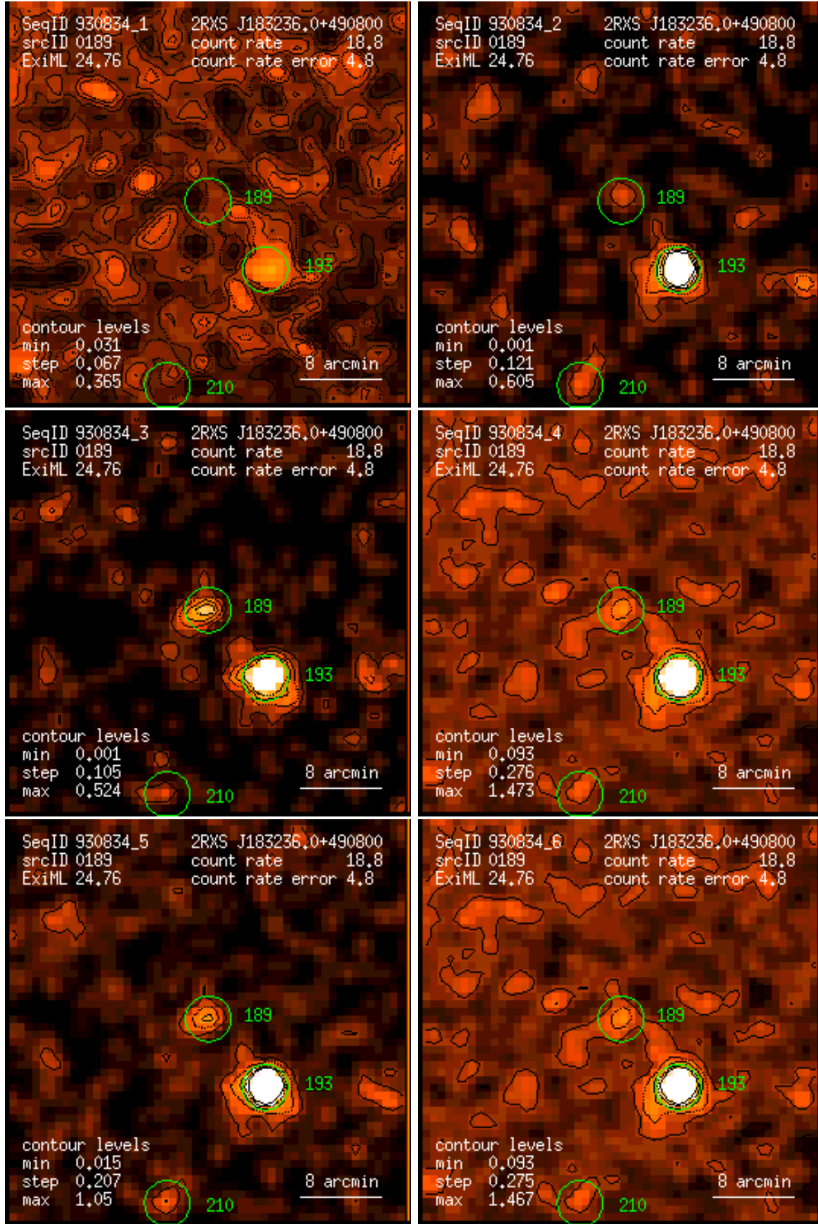
Figure 189: RASS 930834: detection 0189: band rate images, Gaussian filter: (1) PSPC channels 11 – 41, (2) 52 – 90, (3) 91 – 201, (4) 11 – 235, (5) 52 – 201, (6) 11 – 201. Broad band rates in counts/ks. Band rate contour levels in counts/ks/arcmin 2 .
