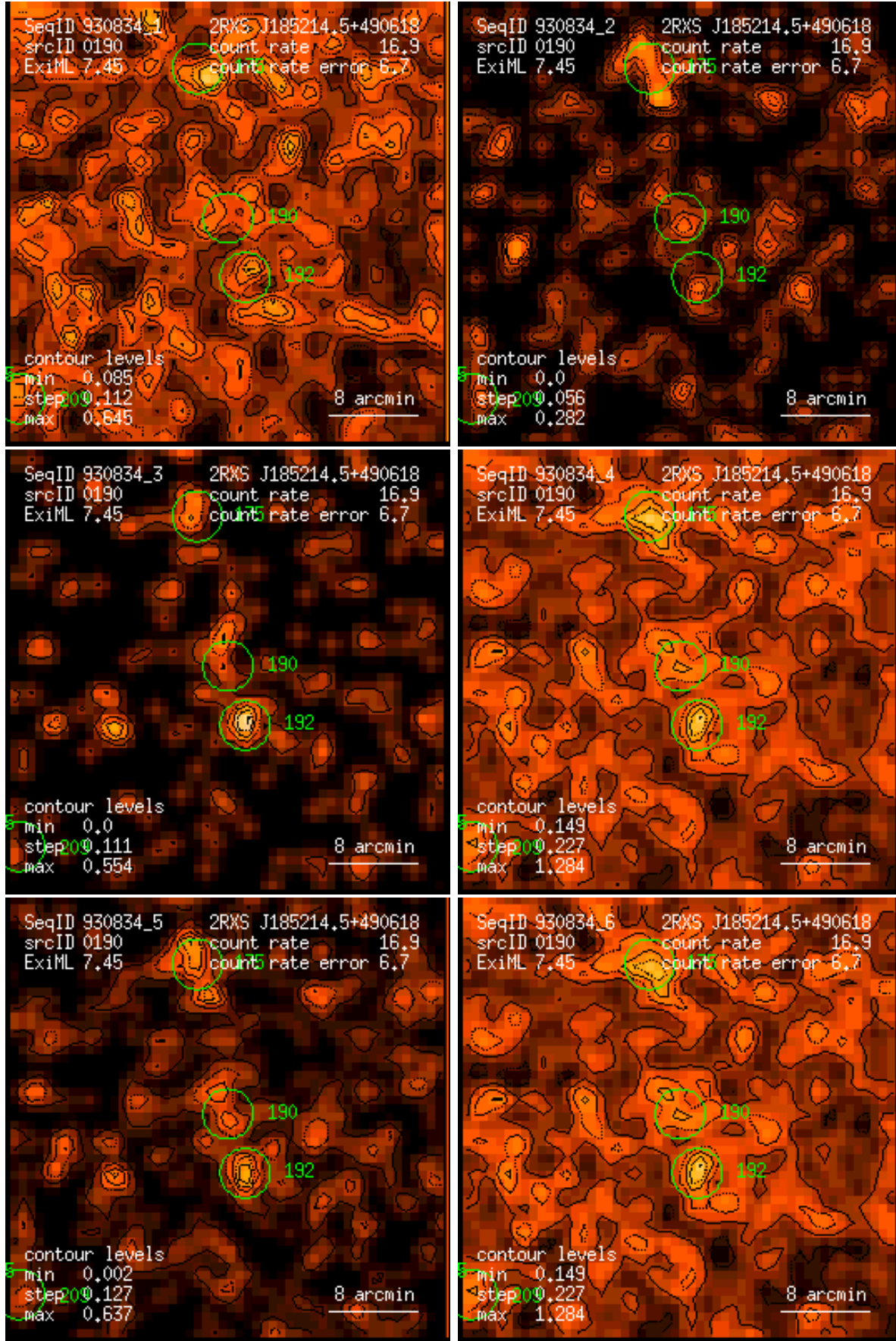
Figure 190: RASS 930834: detection 0190: band rate images, Gaussian filter: (1) PSPC channels 11 – 41, (2) 52 – 90, (3) 91 – 201, (4) 11 – 235, (5) 52 – 201, (6) 11 – 201. Broad band rates in counts/ks. Band rate contour levels in counts/ks/arcmin 2 .
