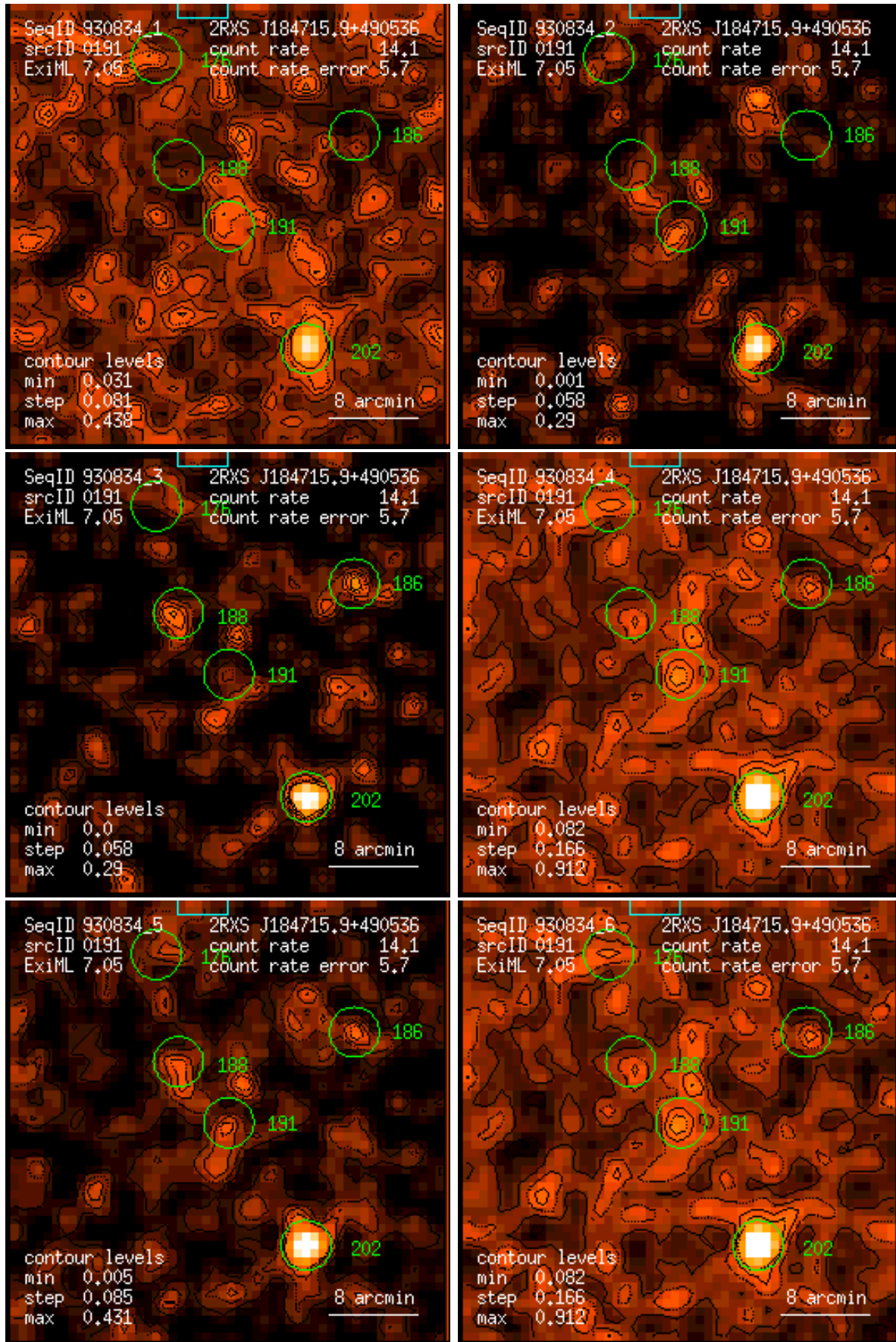
Figure 191: RASS 930834: detection 0191: band rate images, Gaussian filter: (1) PSPC channels 11 – 41, (2) 52 – 90, (3) 91 – 201, (4) 11 – 235, (5) 52 – 201, (6) 11 – 201. Broad band rates in counts/ks. Band rate contour levels in counts/ks/arcmin 2 .
