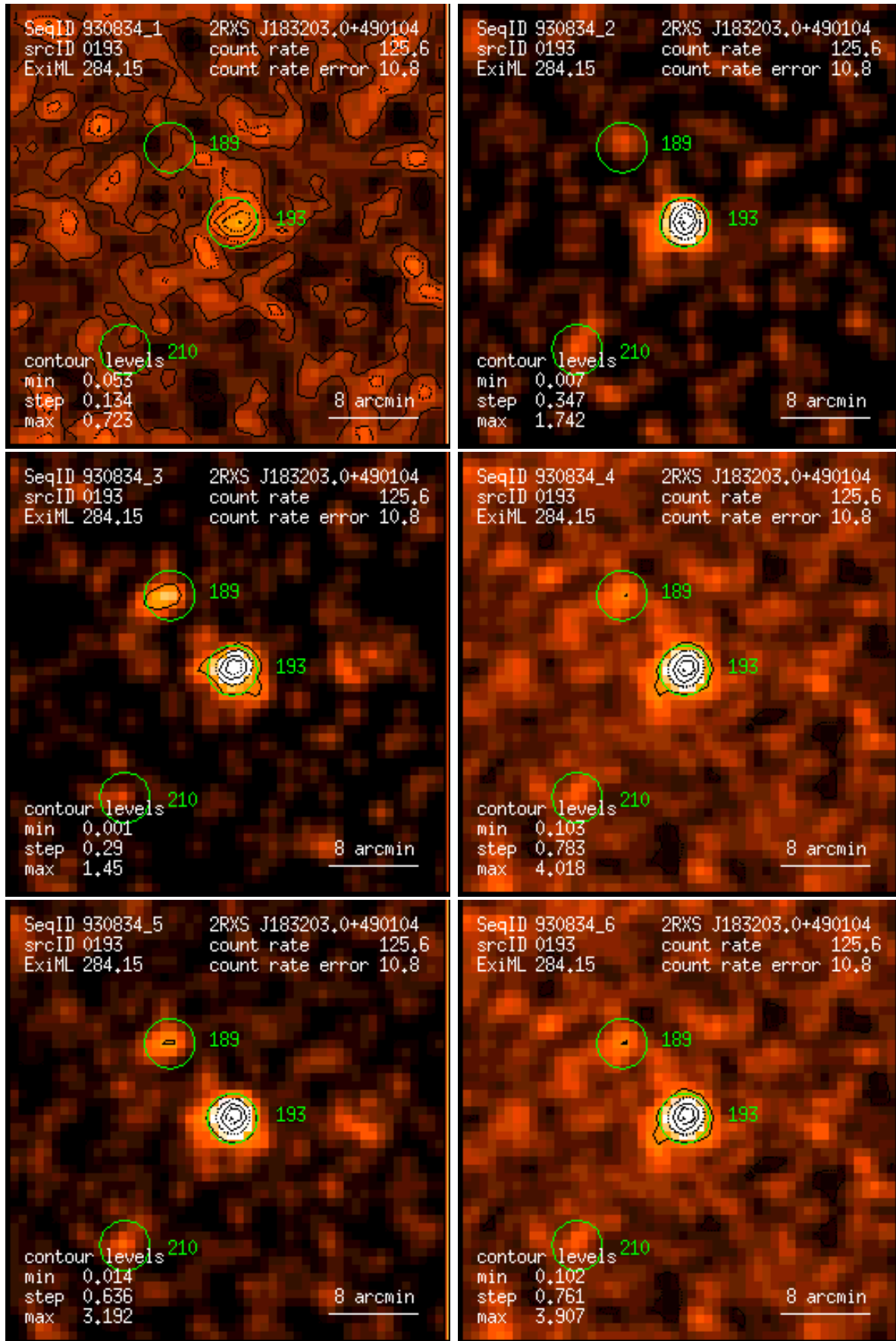
Figure 193: RASS 930834: detection 0193: band rate images, Gaussian filter: (1) PSPC channels 11 – 41, (2) 52 – 90, (3) 91 – 201, (4) 11 – 235, (5) 52 – 201, (6) 11 – 201. Broad band rates in counts/ks. Band rate contour levels in counts/ks/arcmin 2 .
