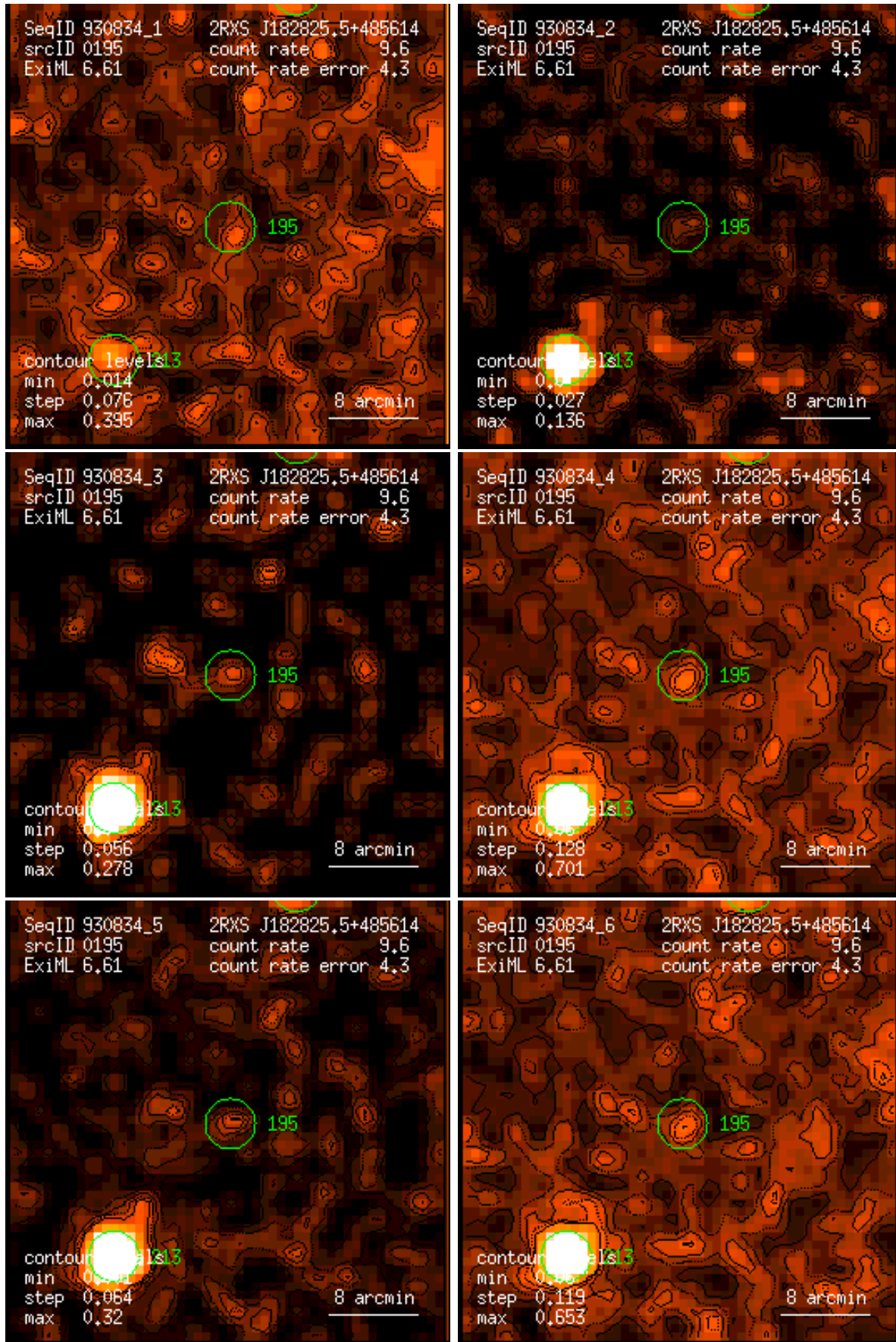
Figure 195: RASS 930834: detection 0195: band rate images, Gaussian filter: (1) PSPC channels 11 – 41, (2) 52 – 90, (3) 91 – 201, (4) 11 – 235, (5) 52 – 201, (6) 11 – 201. Broad band rates in counts/ks. Band rate contour levels in counts/ks/arcmin 2 .
