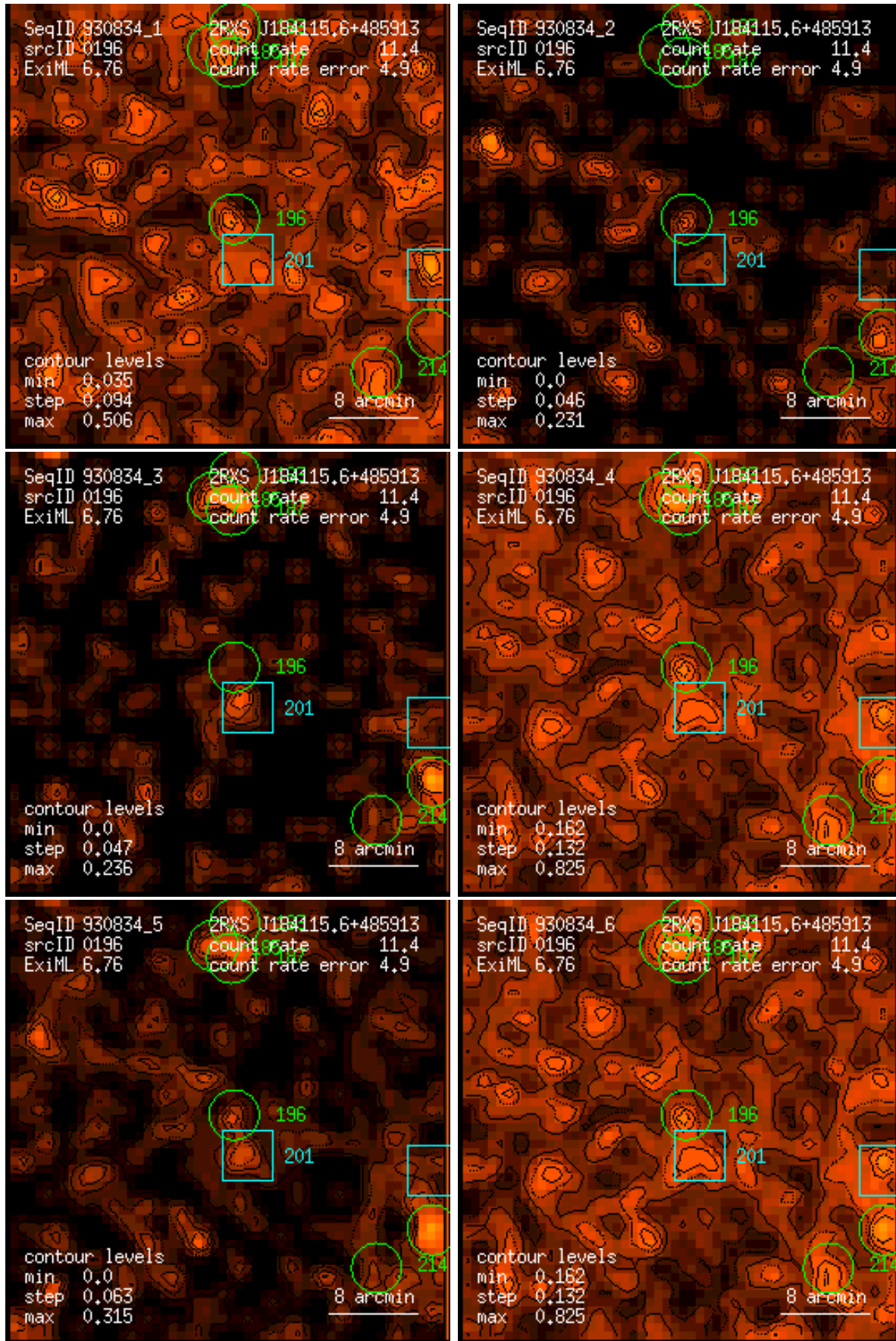
Figure 196: RASS 930834: detection 0196: band rate images, Gaussian filter: (1) PSPC channels 11 – 41, (2) 52 – 90, (3) 91 – 201, (4) 11 – 235, (5) 52 – 201, (6) 11 – 201. Broad band rates in counts/ks. Band rate contour levels in counts/ks/arcmin 2 .
