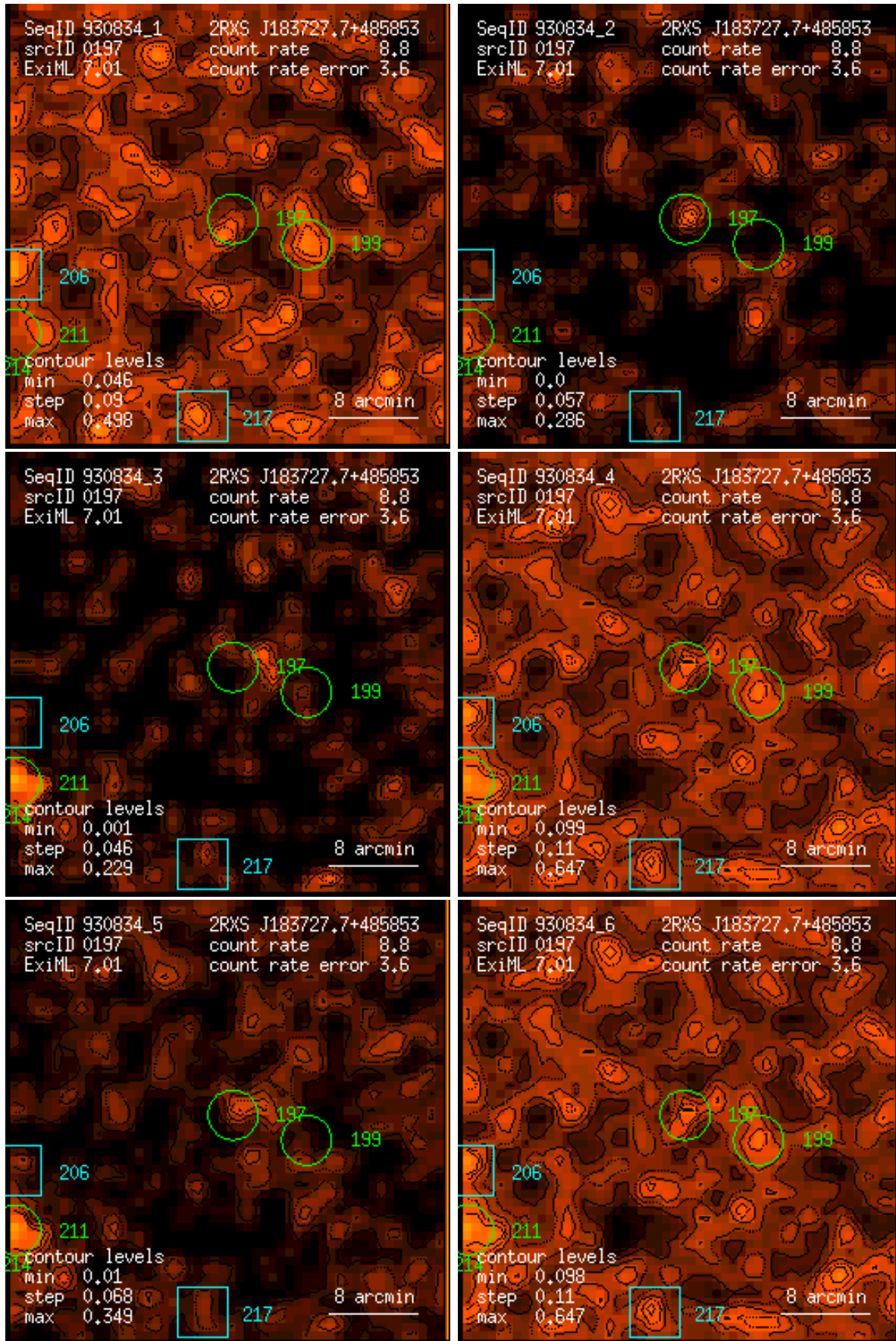
Figure 197: RASS 930834: detection 0197: band rate images, Gaussian filter: (1) PSPC channels 11 – 41, (2) 52 – 90, (3) 91 – 201, (4) 11 – 235, (5) 52 – 201, (6) 11 – 201. Broad band rates in counts/ks. Band rate contour levels in counts/ks/arcmin 2 .
