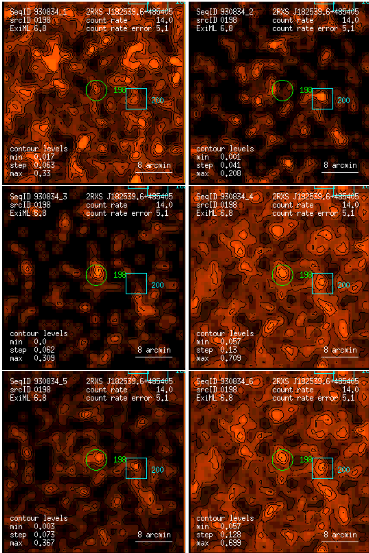
Figure 198: RASS 930834: detection 0198: band rate images, Gaussian filter: (1) PSPC channels 11 – 41, (2) 52 – 90, (3) 91 – 201, (4) 11 – 235, (5) 52 – 201, (6) 11 – 201. Broad band rates in counts/ks. Band rate contour levels in counts/ks/arcmin 2 .
