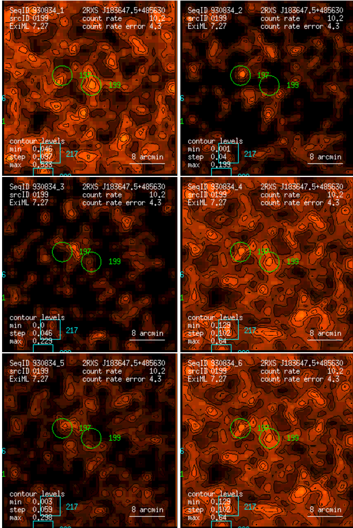
Figure 199: RASS 930834: detection 0199: band rate images, Gaussian filter: (1) PSPC channels 11 – 41, (2) 52 – 90, (3) 91 – 201, (4) 11 – 235, (5) 52 – 201, (6) 11 – 201. Broad band rates in counts/ks. Band rate contour levels in counts/ks/arcmin 2 .
