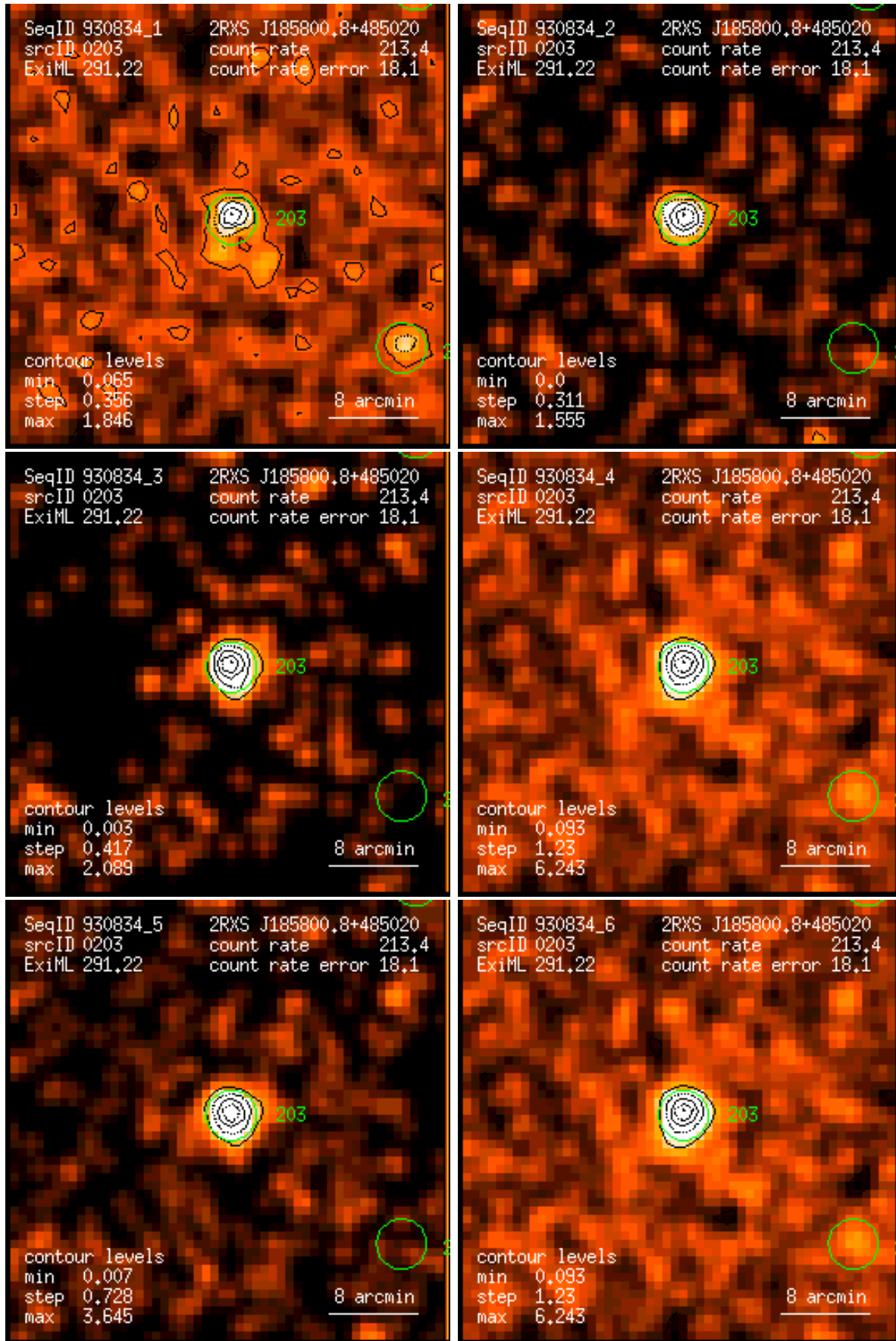
Figure 203: RASS 930834: detection 0203: band rate images, Gaussian filter: (1) PSPC channels 11 – 41, (2) 52 – 90, (3) 91 – 201, (4) 11 – 235, (5) 52 – 201, (6) 11 – 201. Broad band rates in counts/ks. Band rate contour levels in counts/ks/arcmin 2 .
