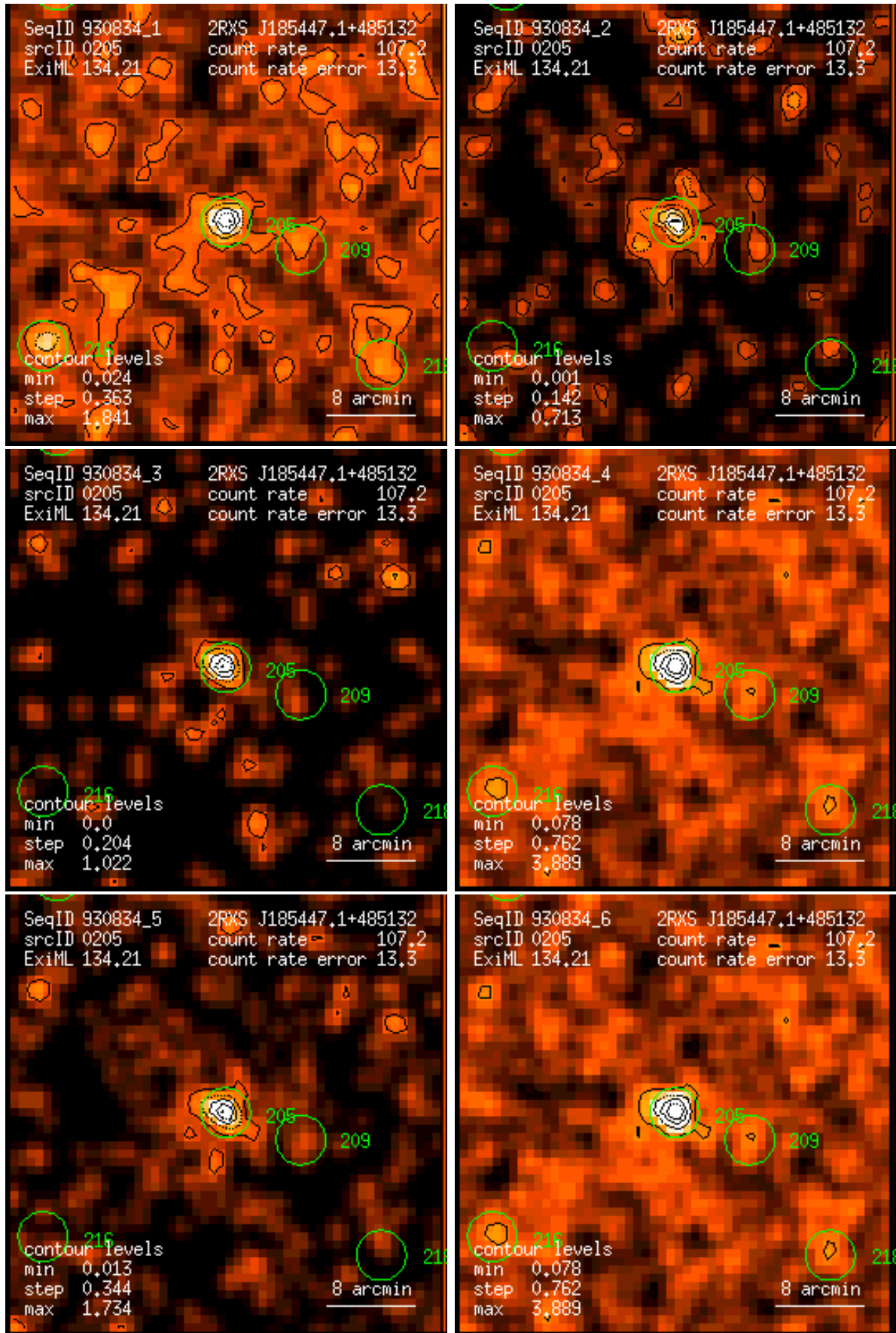
Figure 205: RASS 930834: detection 0205: band rate images, Gaussian filter: (1) PSPC channels 11 – 41, (2) 52 – 90, (3) 91 – 201, (4) 11 – 235, (5) 52 – 201, (6) 11 – 201. Broad band rates in counts/ks. Band rate contour levels in counts/ks/arcmin 2 .
