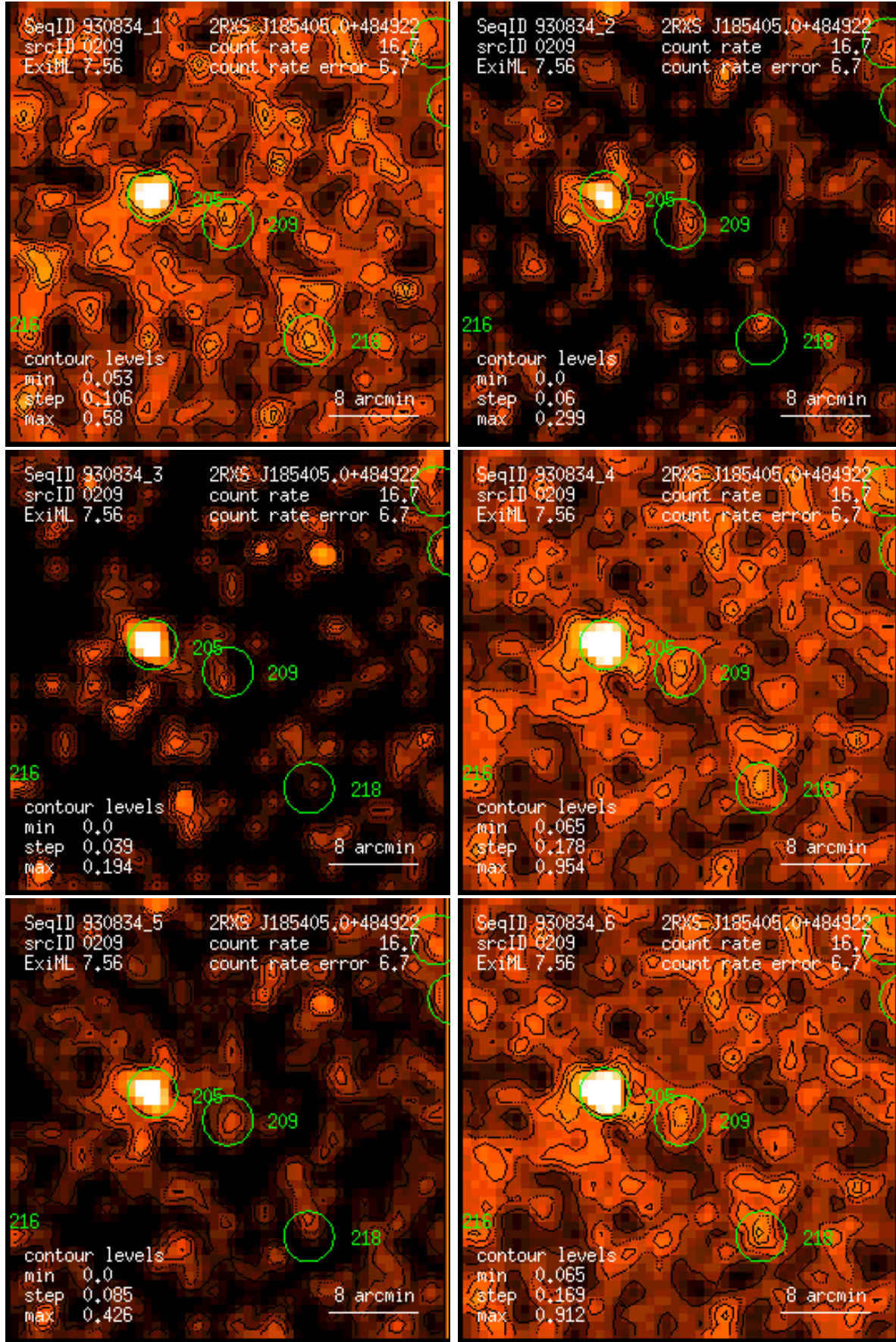
Figure 209: RASS 930834: detection 0209: band rate images, Gaussian filter: (1) PSPC channels 11 – 41, (2) 52 – 90, (3) 91 – 201, (4) 11 – 235, (5) 52 – 201, (6) 11 – 201. Broad band rates in counts/ks. Band rate contour levels in counts/ks/arcmin 2 .
