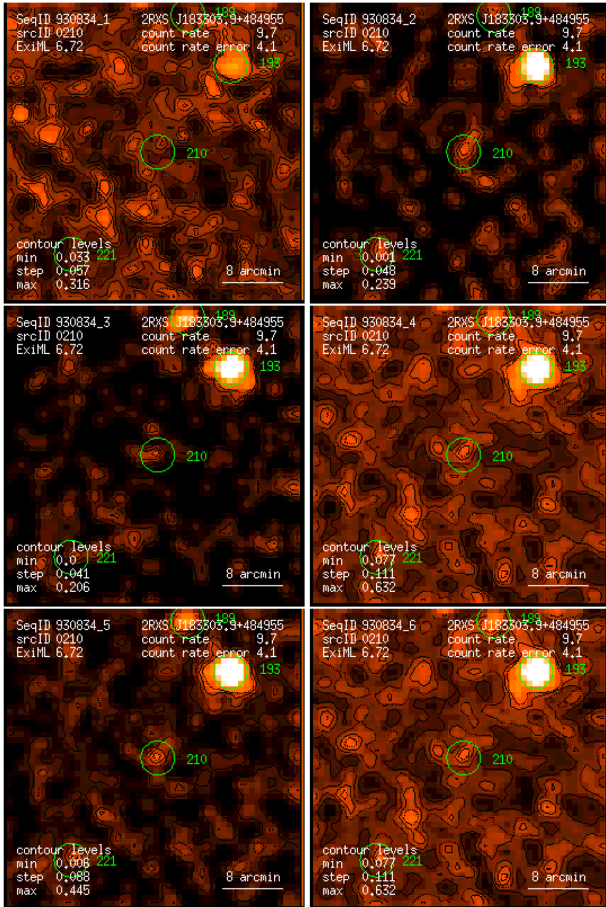
Figure 210: RASS 930834: detection 0210: band rate images, Gaussian filter: (1) PSPC channels 11 – 41, (2) 52 – 90, (3) 91 – 201, (4) 11 – 235, (5) 52 – 201, (6) 11 – 201. Broad band rates in counts/ks. Band rate contour levels in counts/ks/arcmin 2 .
