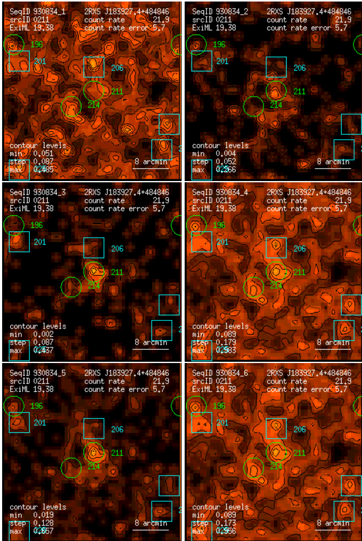
Figure 211: RASS 930834: detection 0211: band rate images, Gaussian filter: (1) PSPC channels 11 – 41, (2) 52 – 90, (3) 91 – 201, (4) 11 – 235, (5) 52 – 201, (6) 11 – 201. Broad band rates in counts/ks. Band rate contour levels in counts/ks/arcmin 2 .
