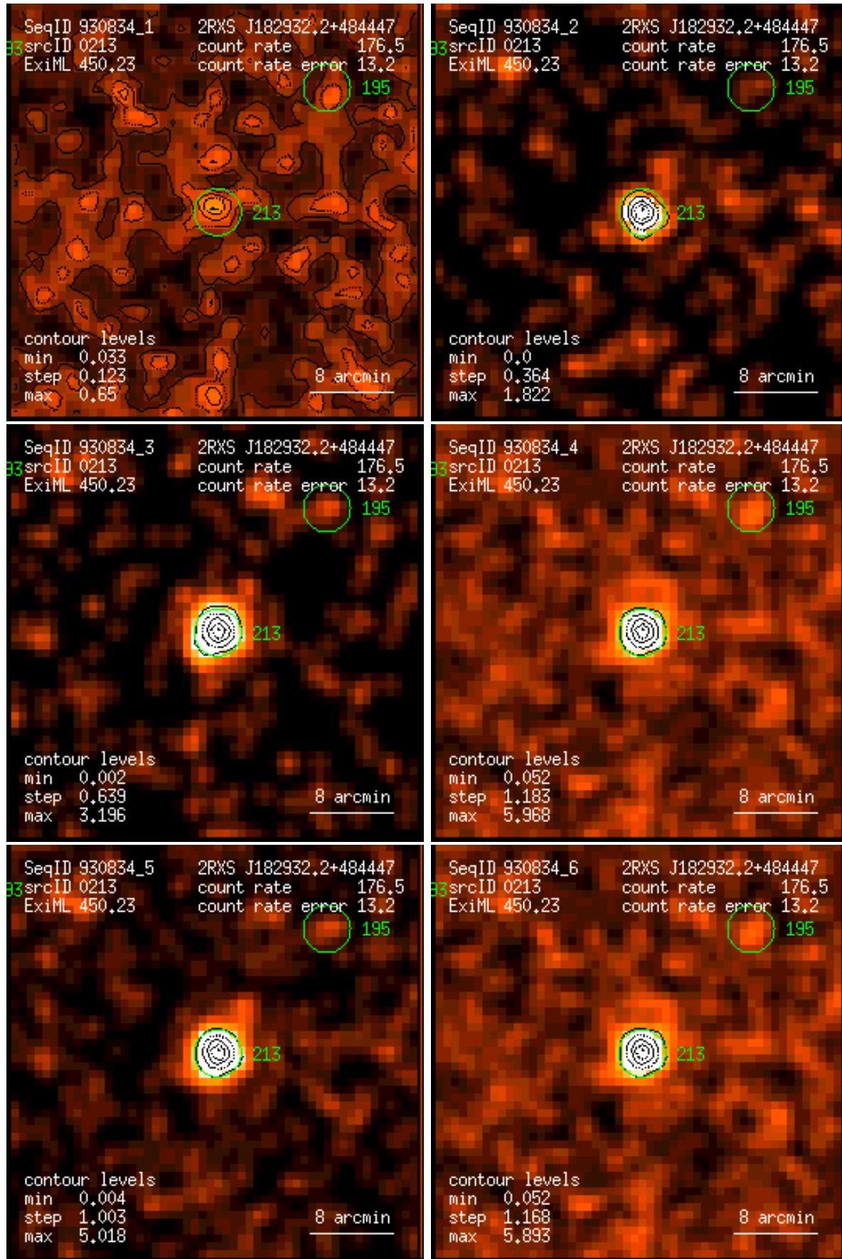
Figure 213: RASS 930834: detection 0213: band rate images, Gaussian filter: (1) PSPC channels 11 – 41, (2) 52 – 90, (3) 91 – 201, (4) 11 – 235, (5) 52 – 201, (6) 11 – 201. Broad band rates in counts/ks. Band rate contour levels in counts/ks/arcmin 2 .
