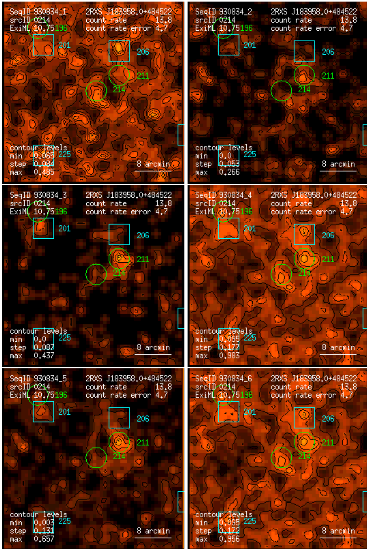
Figure 214: RASS 930834: detection 0214: band rate images, Gaussian filter: (1) PSPC channels 11 – 41, (2) 52 – 90, (3) 91 – 201, (4) 11 – 235, (5) 52 – 201, (6) 11 – 201. Broad band rates in counts/ks. Band rate contour levels in counts/ks/arcmin 2 .
