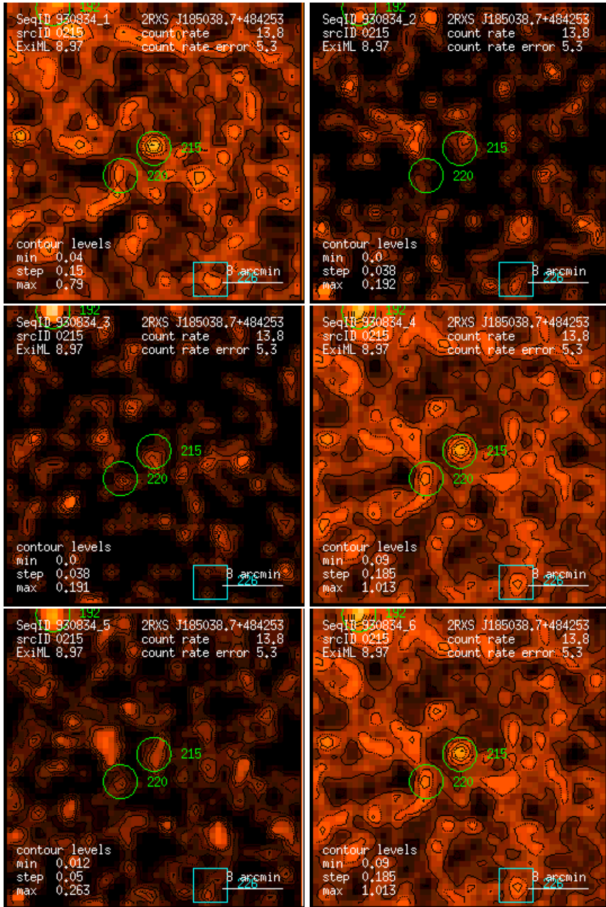
Figure 215: RASS 930834: detection 0215: band rate images, Gaussian filter: (1) PSPC channels 11 – 41, (2) 52 – 90, (3) 91 – 201, (4) 11 – 235, (5) 52 – 201, (6) 11 – 201. Broad band rates in counts/ks. Band rate contour levels in counts/ks/arcmin 2 .
