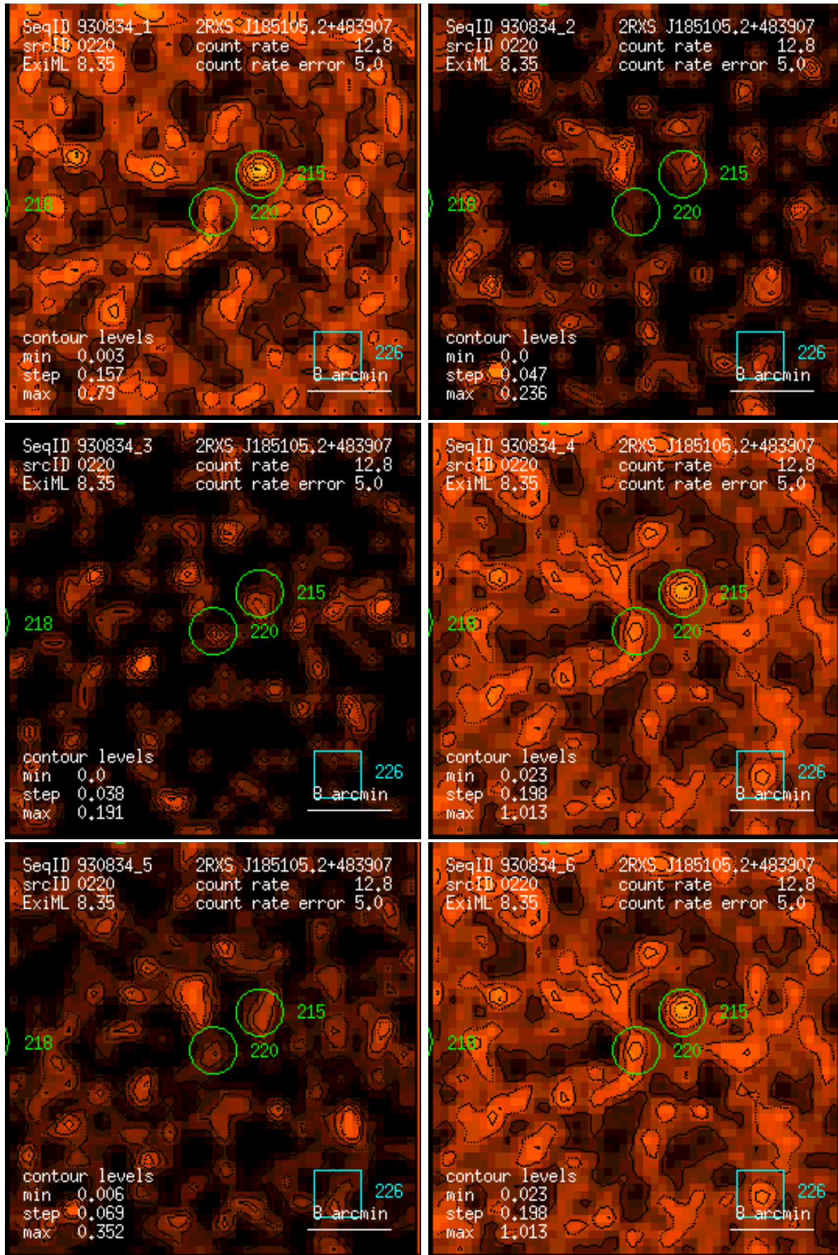
Figure 220: RASS 930834: detection 0220: band rate images, Gaussian filter: (1) PSPC channels 11 – 41, (2) 52 – 90, (3) 91 – 201, (4) 11 – 235, (5) 52 – 201, (6) 11 – 201. Broad band rates in counts/ks. Band rate contour levels in counts/ks/arcmin 2 .
