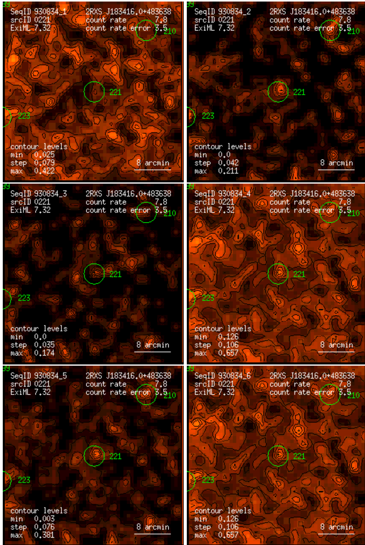
Figure 221: RASS 930834: detection 0221: band rate images, Gaussian filter: (1) PSPC channels 11 – 41, (2) 52 – 90, (3) 91 – 201, (4) 11 – 235, (5) 52 – 201, (6) 11 – 201. Broad band rates in counts/ks. Band rate contour levels in counts/ks/arcmin 2 .
