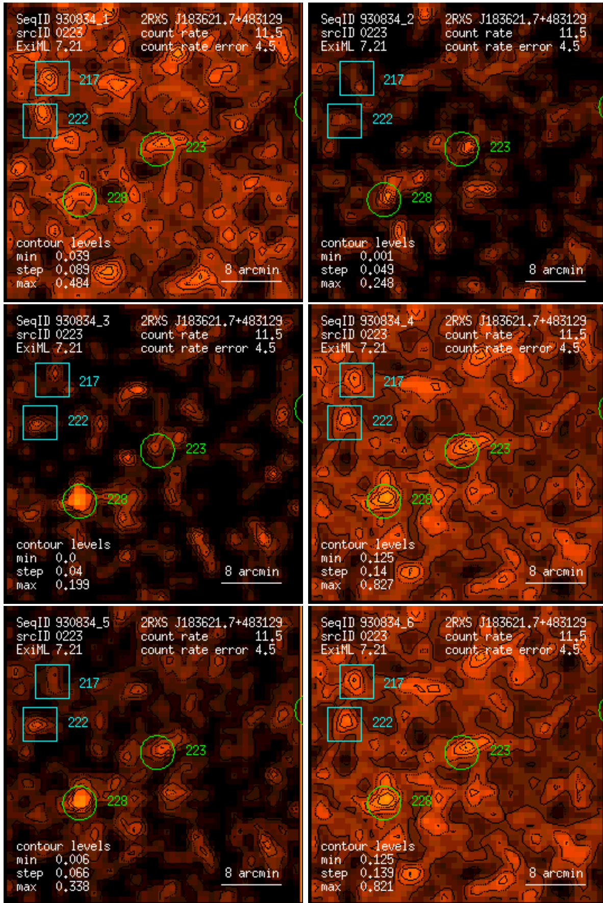
Figure 223: RASS 930834: detection 0223: band rate images, Gaussian filter: (1) PSPC channels 11 – 41, (2) 52 – 90, (3) 91 – 201, (4) 11 – 235, (5) 52 – 201, (6) 11 – 201. Broad band rates in counts/ks. Band rate contour levels in counts/ks/arcmin 2 .
