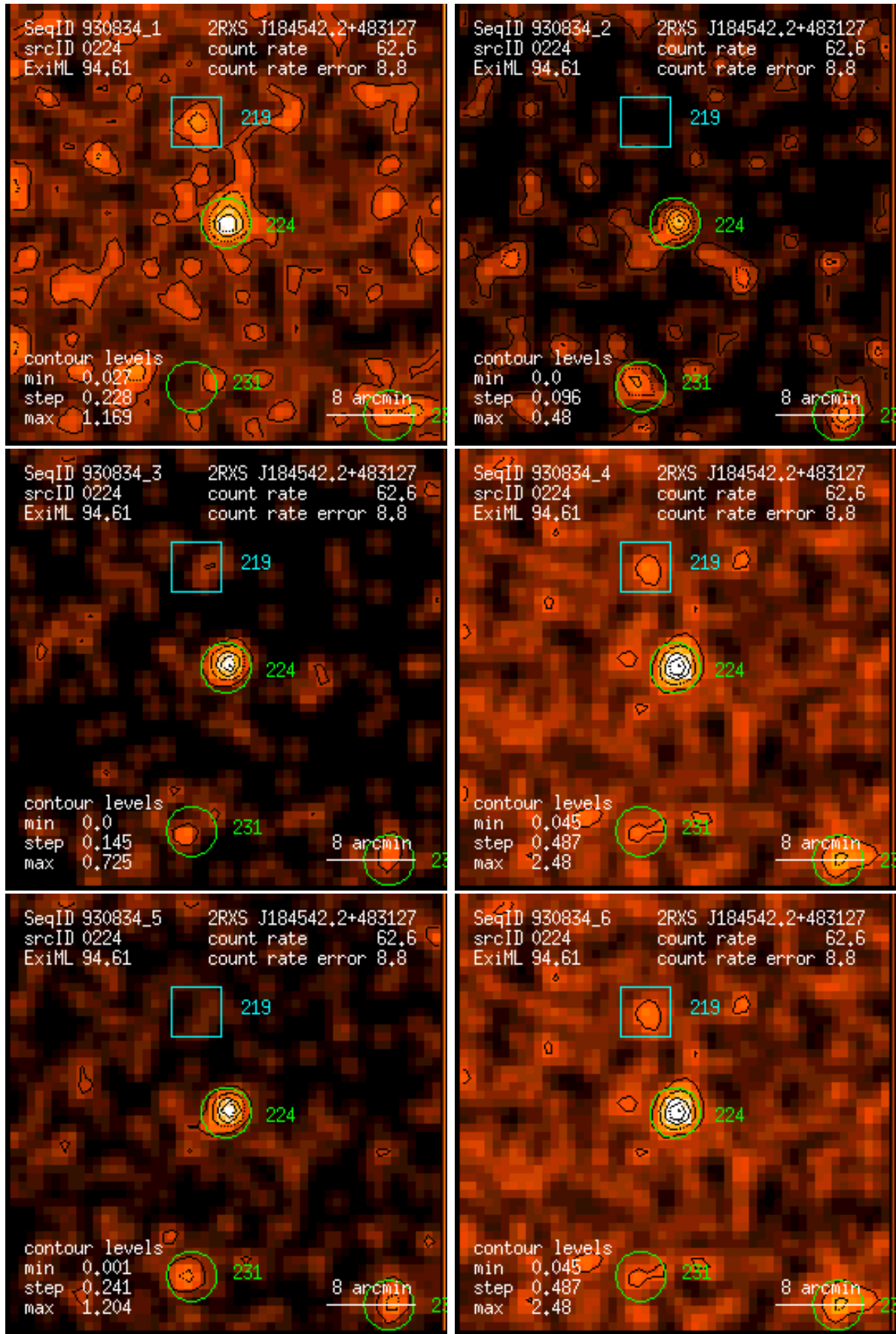
Figure 224: RASS 930834: detection 0224: band rate images, Gaussian filter: (1) PSPC channels 11 – 41, (2) 52 – 90, (3) 91 – 201, (4) 11 – 235, (5) 52 – 201, (6) 11 – 201. Broad band rates in counts/ks. Band rate contour levels in counts/ks/arcmin 2 .
