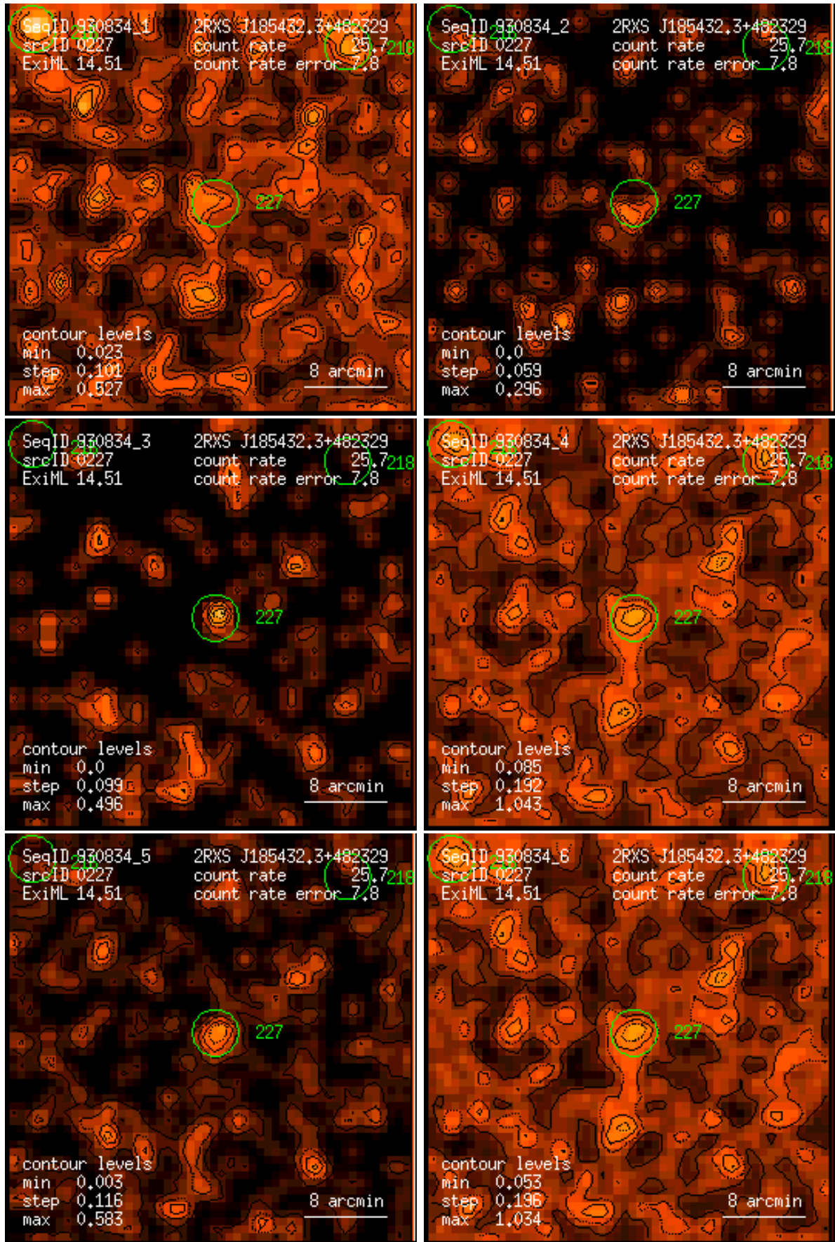
Figure 227: RASS 930834: detection 0227: band rate images, Gaussian filter: (1) PSPC channels 11 – 41, (2) 52 – 90, (3) 91 – 201, (4) 11 – 235, (5) 52 – 201, (6) 11 – 201. Broad band rates in counts/ks. Band rate contour levels in counts/ks/arcmin 2 .
