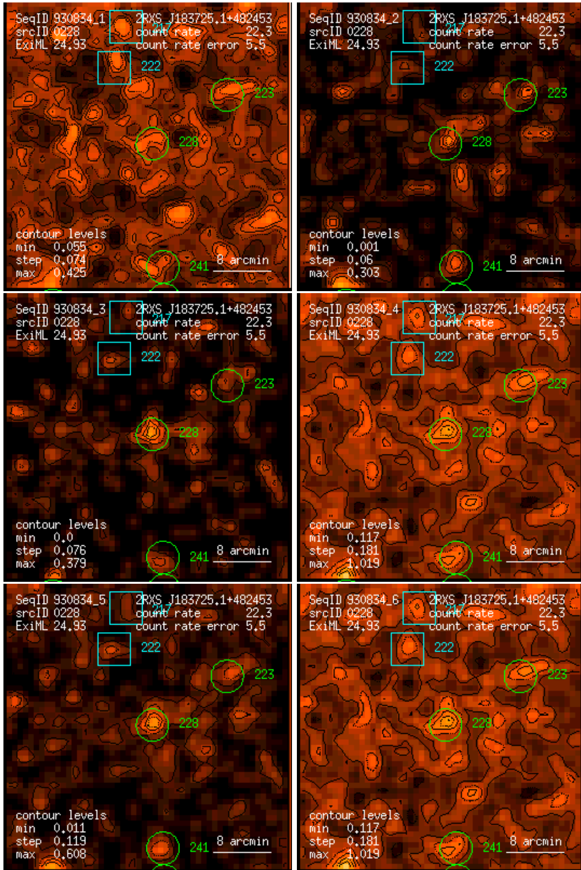
Figure 228: RASS 930834: detection 0228: band rate images, Gaussian filter: (1) PSPC channels 11 – 41, (2) 52 – 90, (3) 91 – 201, (4) 11 – 235, (5) 52 – 201, (6) 11 – 201. Broad band rates in counts/ks. Band rate contour levels in counts/ks/arcmin 2 .
