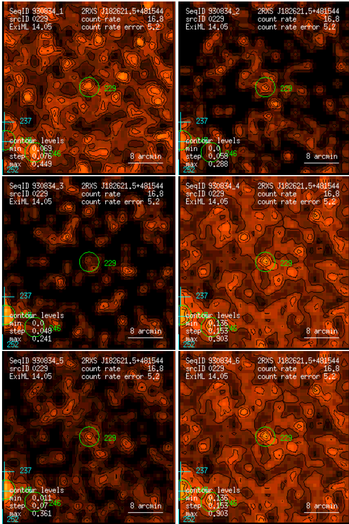
Figure 229: RASS 930834: detection 0229: band rate images, Gaussian filter: (1) PSPC channels 11 – 41, (2) 52 – 90, (3) 91 – 201, (4) 11 – 235, (5) 52 – 201, (6) 11 – 201. Broad band rates in counts/ks. Band rate contour levels in counts/ks/arcmin 2 .
