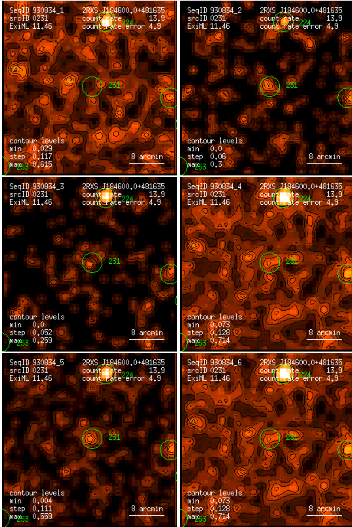
Figure 231: RASS 930834: detection 0231: band rate images, Gaussian filter: (1) PSPC channels 11 – 41, (2) 52 – 90, (3) 91 – 201, (4) 11 – 235, (5) 52 – 201, (6) 11 – 201. Broad band rates in counts/ks. Band rate contour levels in counts/ks/arcmin 2 .
