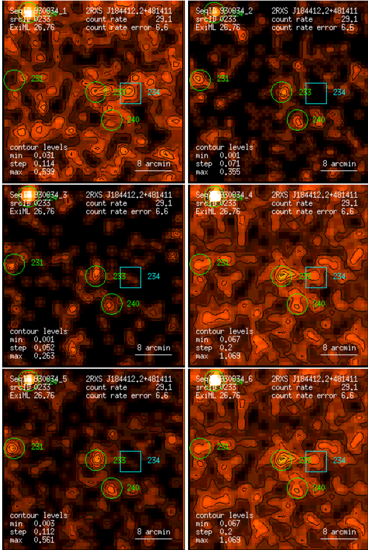
Figure 233: RASS 930834: detection 0233: band rate images, Gaussian filter: (1) PSPC channels 11 – 41, (2) 52 – 90, (3) 91 – 201, (4) 11 – 235, (5) 52 – 201, (6) 11 – 201. Broad band rates in counts/ks. Band rate contour levels in counts/ks/arcmin 2 .
