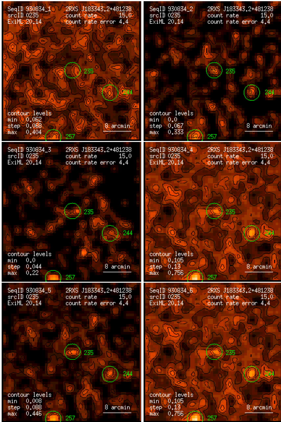
Figure 235: RASS 930834: detection 0235: band rate images, Gaussian filter: (1) PSPC channels 11 – 41, (2) 52 – 90, (3) 91 – 201, (4) 11 – 235, (5) 52 – 201, (6) 11 – 201. Broad band rates in counts/ks. Band rate contour levels in counts/ks/arcmin 2 .
