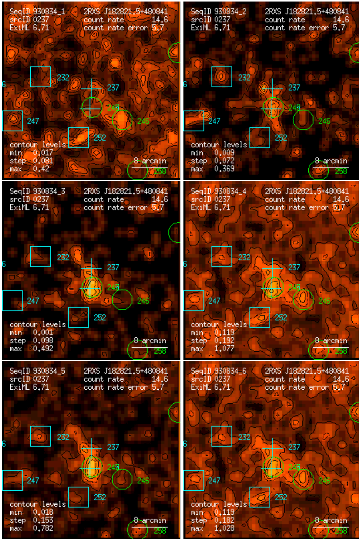
Figure 237: RASS 930834: detection 0237: band rate images, Gaussian filter: (1) PSPC channels 11 – 41, (2) 52 – 90, (3) 91 – 201, (4) 11 – 235, (5) 52 – 201, (6) 11 – 201. Broad band rates in counts/ks. Band rate contour levels in counts/ks/arcmin 2 .
