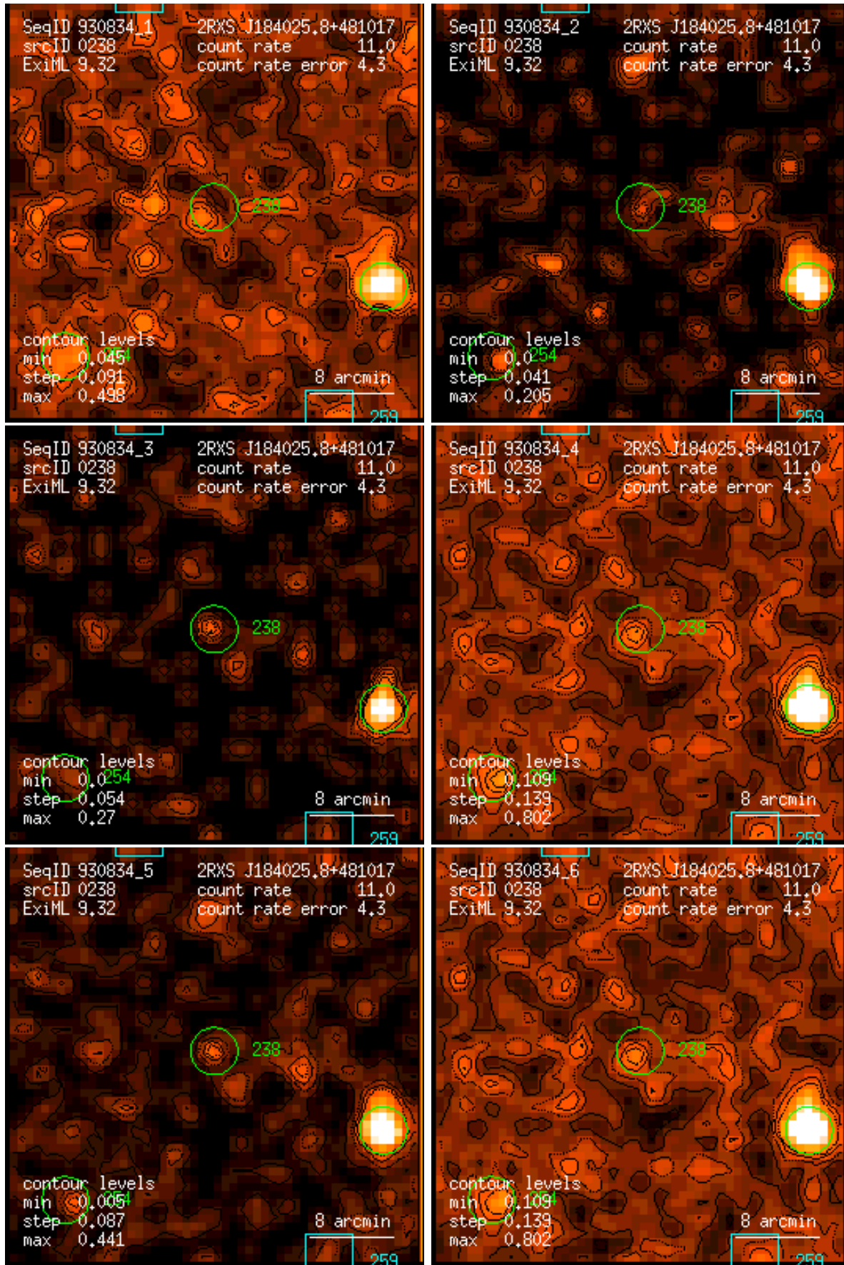
Figure 238: RASS 930834: detection 0238: band rate images, Gaussian filter: (1) PSPC channels 11 – 41, (2) 52 – 90, (3) 91 – 201, (4) 11 – 235, (5) 52 – 201, (6) 11 – 201. Broad band rates in counts/ks. Band rate contour levels in counts/ks/arcmin 2 .
