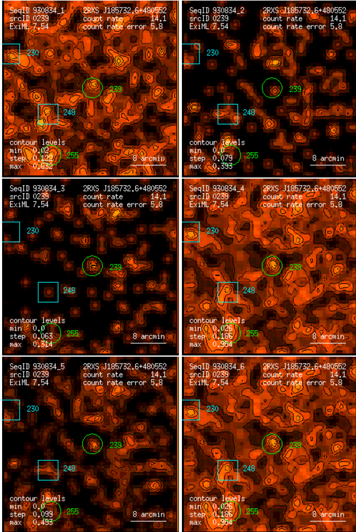
Figure 239: RASS 930834: detection 0239: band rate images, Gaussian filter: (1) PSPC channels 11 – 41, (2) 52 – 90, (3) 91 – 201, (4) 11 – 235, (5) 52 – 201, (6) 11 – 201. Broad band rates in counts/ks. Band rate contour levels in counts/ks/arcmin 2 .
