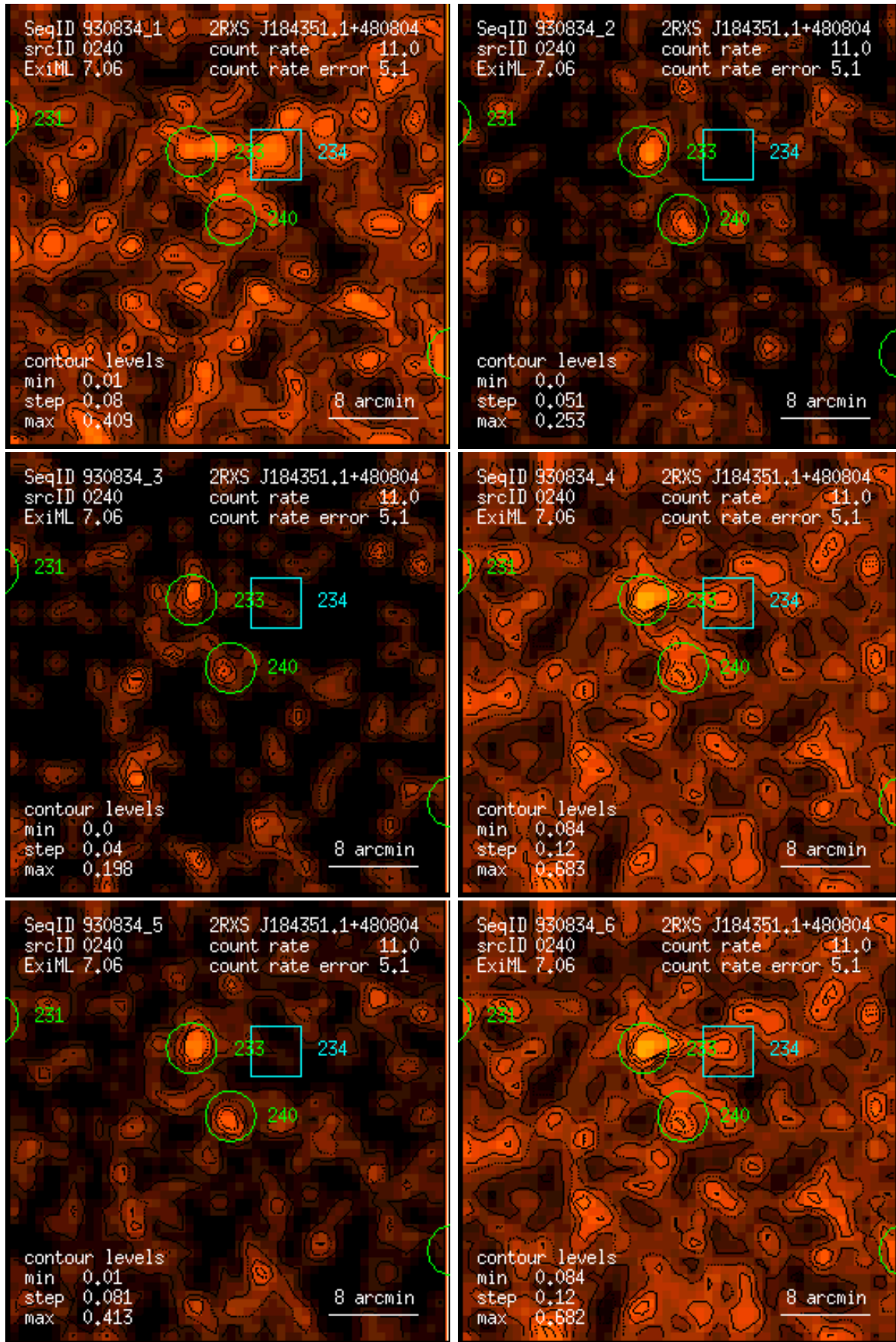
Figure 240: RASS 930834: detection 0240: band rate images, Gaussian filter: (1) PSPC channels 11 – 41, (2) 52 – 90, (3) 91 – 201, (4) 11 – 235, (5) 52 – 201, (6) 11 – 201. Broad band rates in counts/ks. Band rate contour levels in counts/ks/arcmin 2 .
