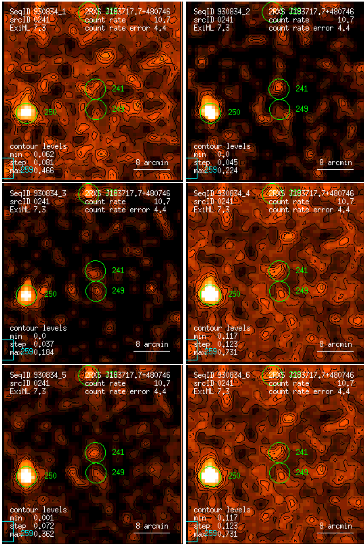
Figure 241: RASS 930834: detection 0241: band rate images, Gaussian filter: (1) PSPC channels 11 – 41, (2) 52 – 90, (3) 91 – 201, (4) 11 – 235, (5) 52 – 201, (6) 11 – 201. Broad band rates in counts/ks. Band rate contour levels in counts/ks/arcmin 2 .
