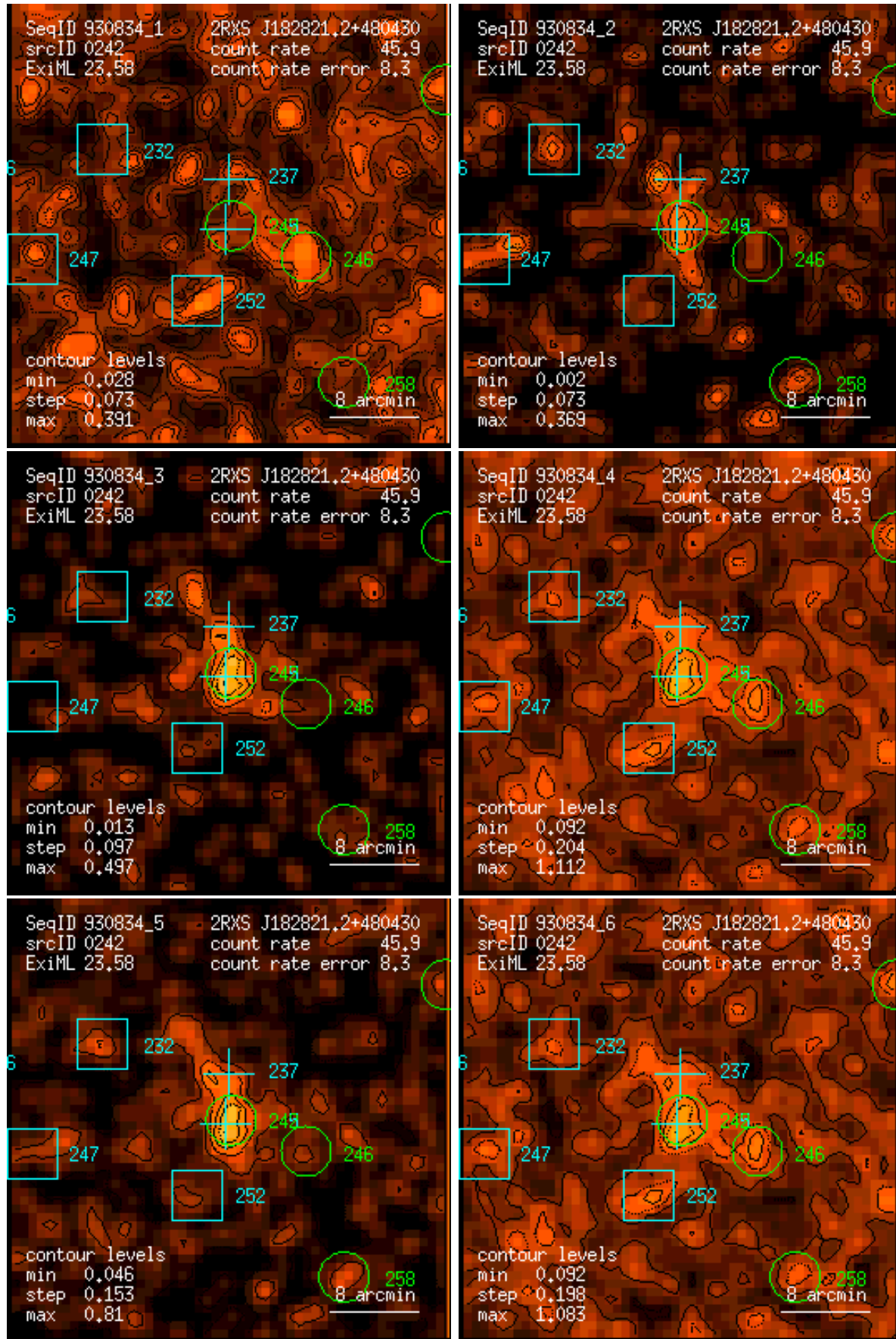
Figure 242: RASS 930834: detection 0242: band rate images, Gaussian filter: (1) PSPC channels 11 – 41, (2) 52 – 90, (3) 91 – 201, (4) 11 – 235, (5) 52 – 201, (6) 11 – 201. Broad band rates in counts/ks. Band rate contour levels in counts/ks/arcmin 2 .
