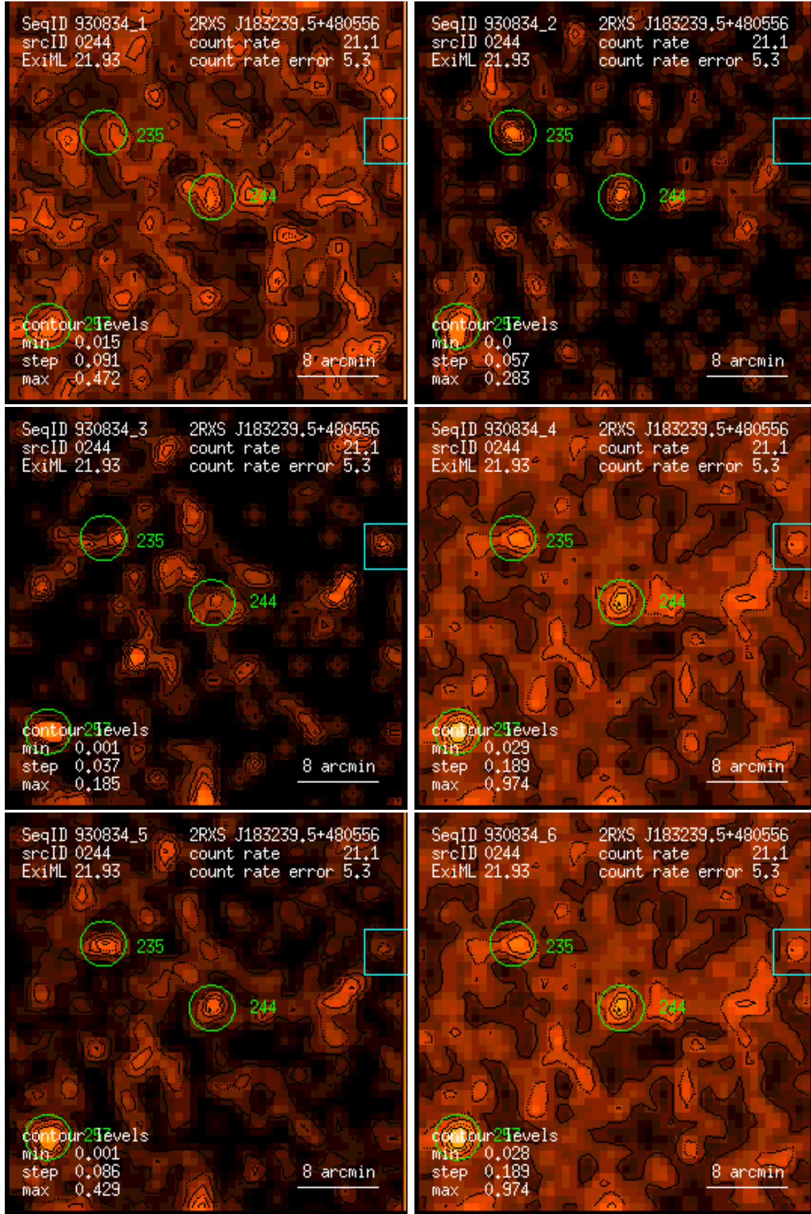
Figure 244: RASS 930834: detection 0244: band rate images, Gaussian filter: (1) PSPC channels 11 – 41, (2) 52 – 90, (3) 91 – 201, (4) 11 – 235, (5) 52 – 201, (6) 11 – 201. Broad band rates in counts/ks. Band rate contour levels in counts/ks/arcmin 2 .
