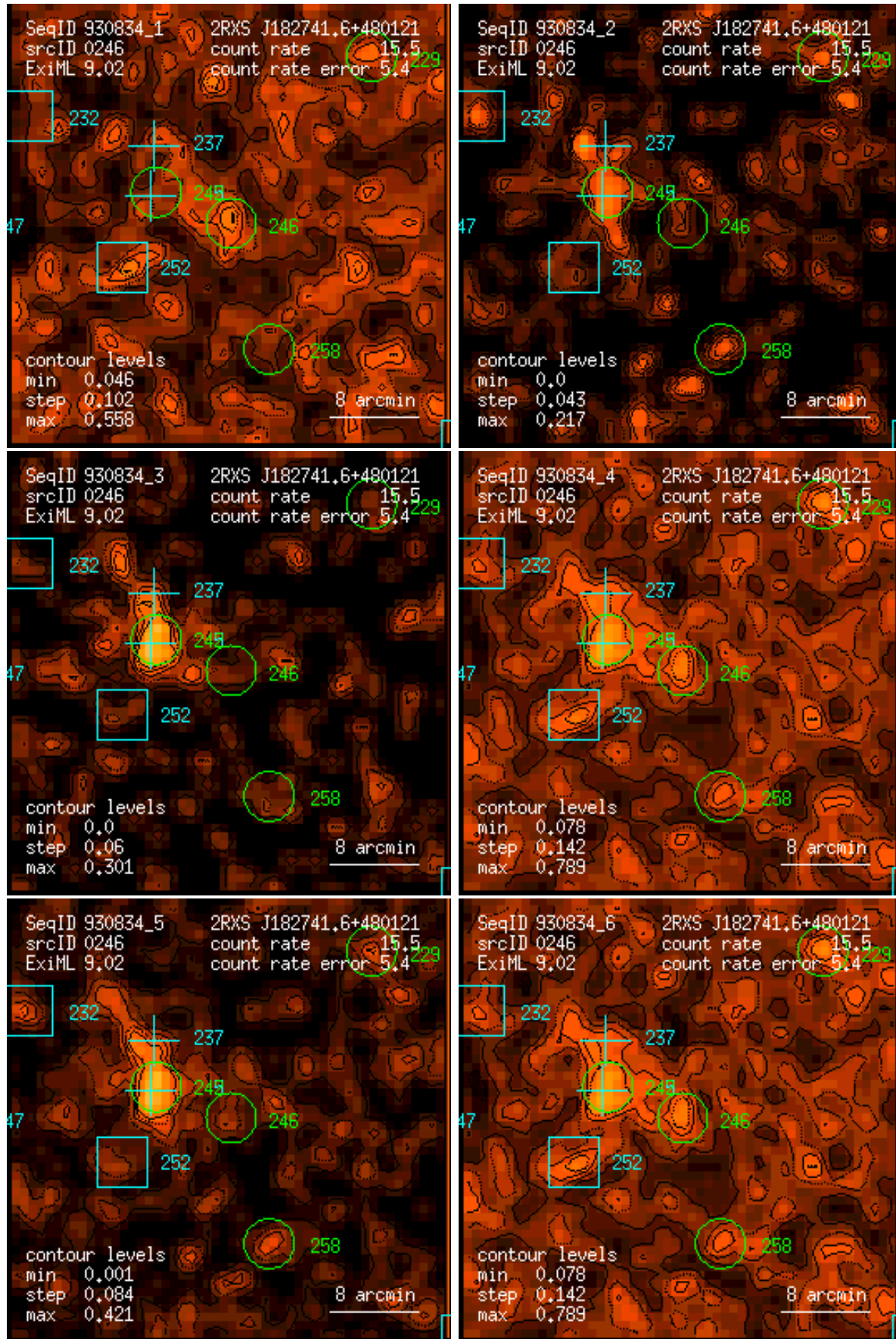
Figure 246: RASS 930834: detection 0246: band rate images, Gaussian filter: (1) PSPC channels 11 – 41, (2) 52 – 90, (3) 91 – 201, (4) 11 – 235, (5) 52 – 201, (6) 11 – 201. Broad band rates in counts/ks. Band rate contour levels in counts/ks/arcmin 2 .
