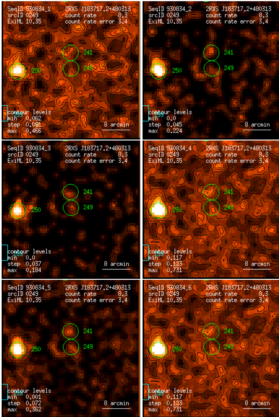
Figure 249: RASS 930834: detection 0249: band rate images, Gaussian filter: (1) PSPC channels 11 – 41, (2) 52 – 90, (3) 91 – 201, (4) 11 – 235, (5) 52 – 201, (6) 11 – 201. Broad band rates in counts/ks. Band rate contour levels in counts/ks/arcmin 2 .
