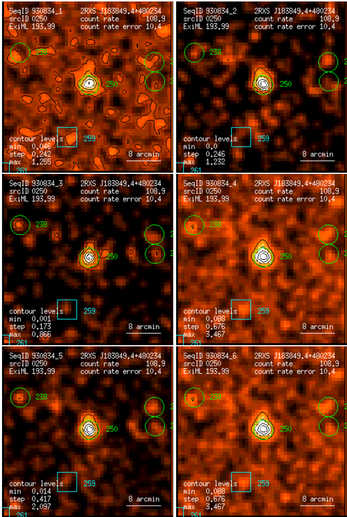
Figure 250: RASS 930834: detection 0250: band rate images, Gaussian filter: (1) PSPC channels 11 – 41, (2) 52 – 90, (3) 91 – 201, (4) 11 – 235, (5) 52 – 201, (6) 11 – 201. Broad band rates in counts/ks. Band rate contour levels in counts/ks/arcmin 2 .
