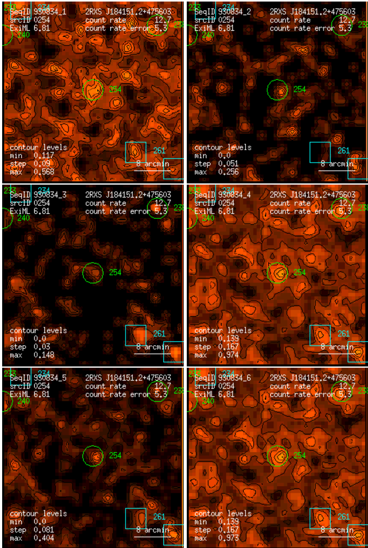
Figure 254: RASS 930834: detection 0254: band rate images, Gaussian filter: (1) PSPC channels 11 – 41, (2) 52 – 90, (3) 91 – 201, (4) 11 – 235, (5) 52 – 201, (6) 11 – 201. Broad band rates in counts/ks. Band rate contour levels in counts/ks/arcmin 2 .
