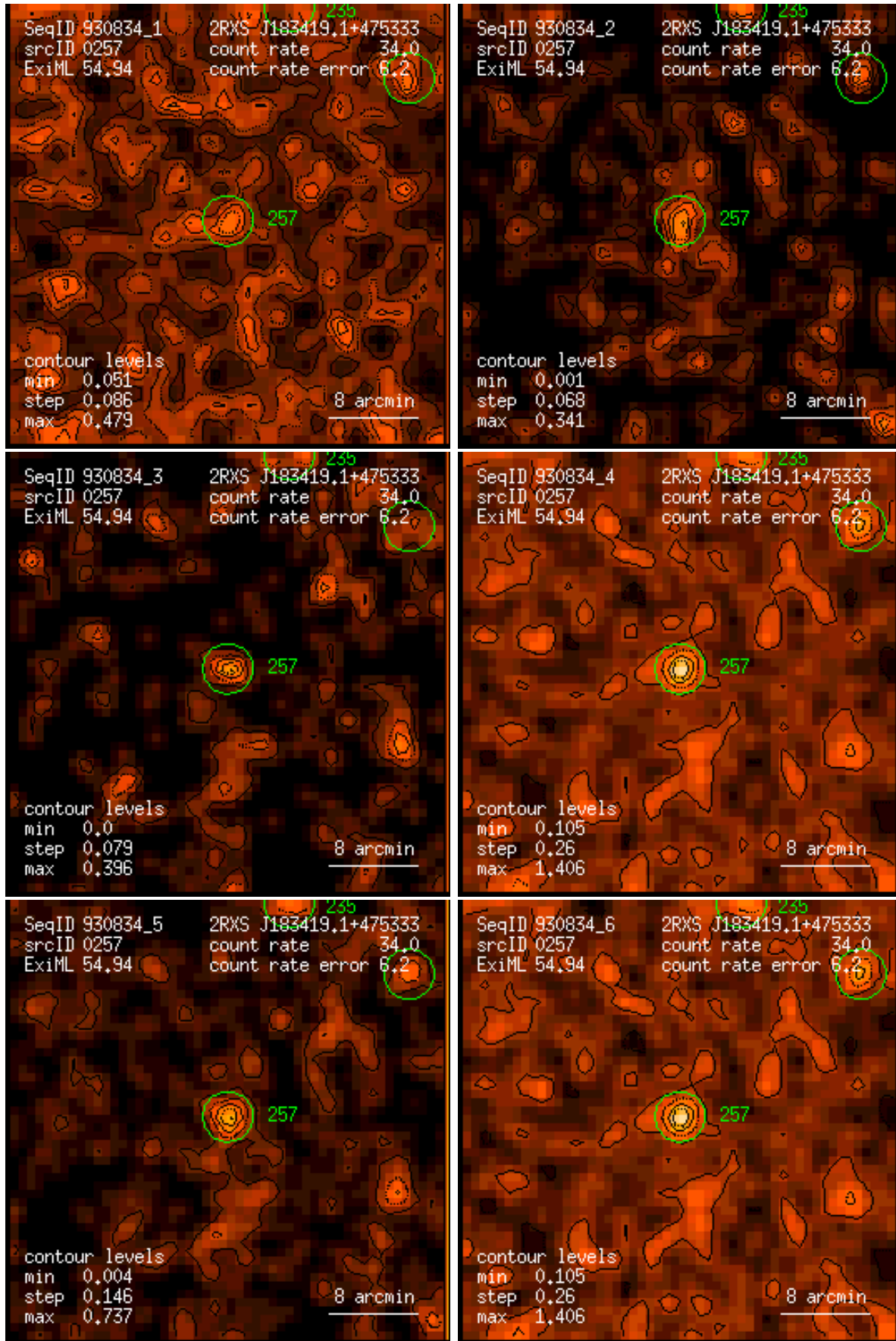
Figure 257: RASS 930834: detection 0257: band rate images, Gaussian filter: (1) PSPC channels 11 – 41, (2) 52 – 90, (3) 91 – 201, (4) 11 – 235, (5) 52 – 201, (6) 11 – 201. Broad band rates in counts/ks. Band rate contour levels in counts/ks/arcmin 2 .
